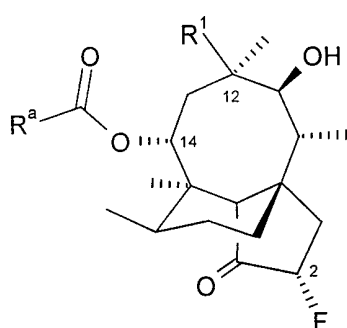
(2 S )-2-Fluoro
