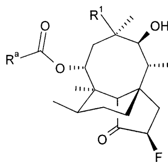
(2 R )-2-Fluoro
