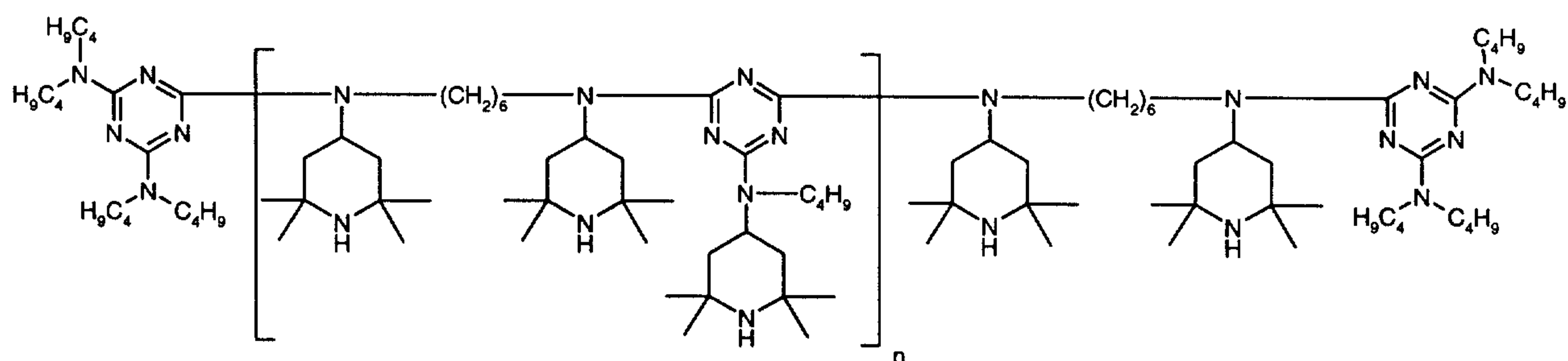
Chimassorb® 2020 (H10)
