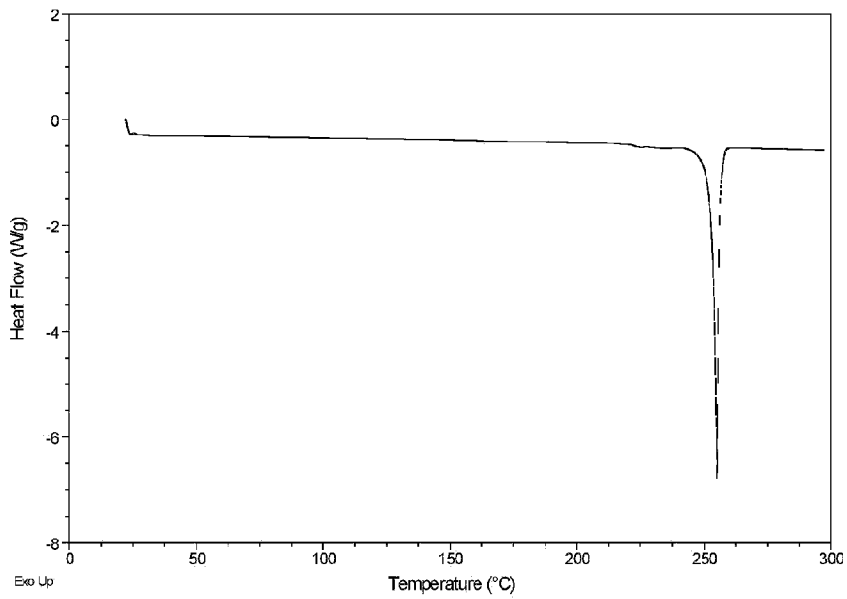
FIG. 2 DSC trace for Example 4 – Form A
