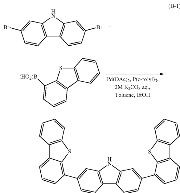
Step 2: Synthesis of 2,7-di-(dibenzothiophen-4-yl)-9-phenyl-9H-carbazole (abbreviated as 2,7DBT2PC-II)
