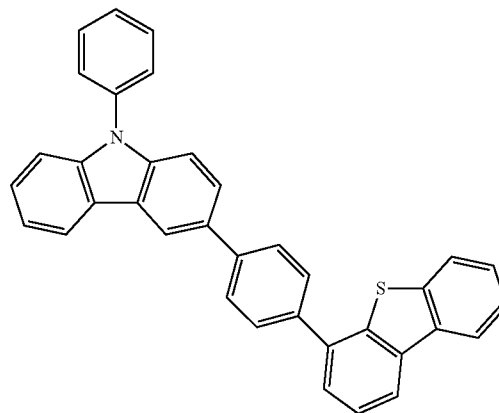
Synthesis Method of 3-[4-(dibenzothiophen-4-yl)-phenyl]-9-phenyl-9H-carbazole (abbreviated as DBTPPC-II)
