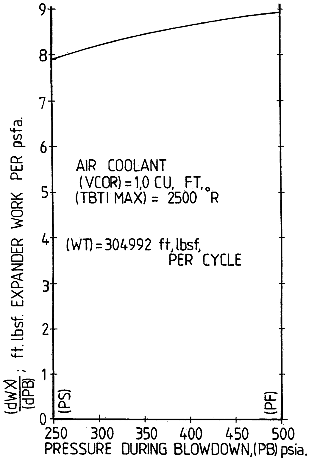
FIGURE 29 EXPANDER ENGINE WORK OUTPUT PER BLOWDOWN CYCLE
