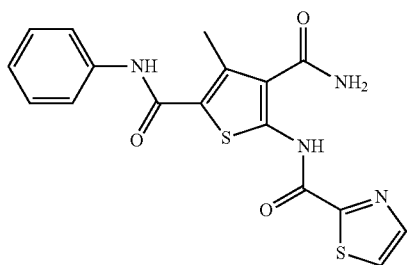
3-Methyl-N2-phenyl-5-(thiazole-2-carboxamido) thiophene-2,4-dicarboxamide (ZW-1053)
