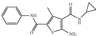
5-Amino-N4-cyclopropyl-3-methyl-N2-phenylthiophene-2,4-dicarboxamide (ZW-792)
