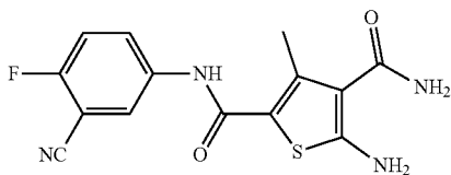
5-Amino-N2-(3-cyano-4-fluorophenyl)-3-methylthiophene-2,4-dicarboxamide (ZW-1039)
