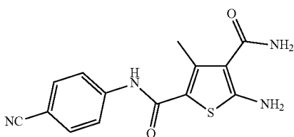
5-Amino-N2-(4-cyanophenyl)-3-methylthiophene-2,4-dicarboxamide (ZW-1038)
