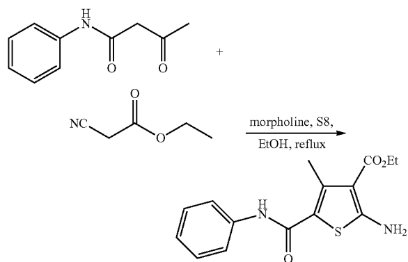
Ethyl 2-amino-4-methyl-5-(phenylcarbamoyl)thiophene-3-carboxylate. (ZW-1045)
