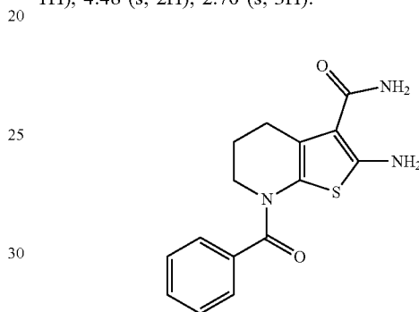
2-Amino-7-benzoyl-4,5,6,7-tetrahydrothieno [2,3-b]pyridine-3-carboxamide (ZW-1071)
