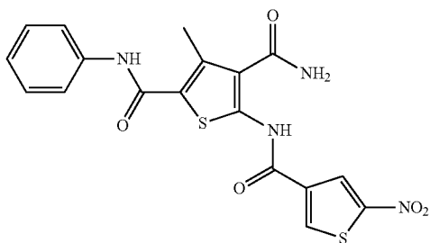
3-Methyl-5-(5-nitrothiophene-3-carboxamido)-N2- phenylthiophene-2,4-dicarboxamide (ZW-1054)
