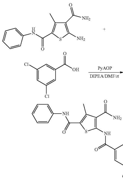
5-(3,5-Dichlorobenzamido)-3-methyl-N2-phenylthiophene-2,4-dicarboxamide (ZW-1040)
