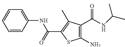
5-Amino-3-methyl-N2-phenylthiophene-2,4-dicarboxamide (ZW-793)
