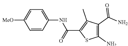
5-Amino-N2-(4-methoxyphenyl)-3-methylthiophene-2,4-dicarboxamide (ZW-769)
