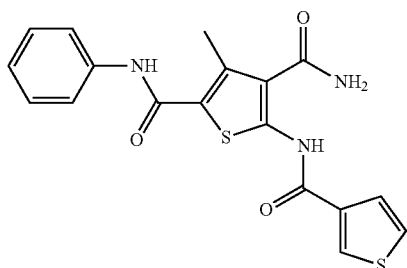
3-Methyl-N2-phenyl-5-(thiophene-3-carboxamido) thiophene-2,4-dicarboxamide (ZW-1055)
