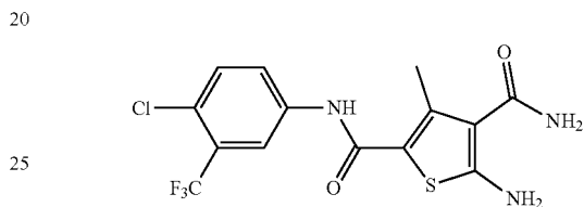
5-Amino-N2-(4-chloro-3-(trifluoromethyl)phenyl)-3-methylthiophene-2,4-dicarboxamide (ZW-1067)
