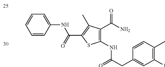
5-(2-(3-Fluoro-4-methylphenyl)acetamido)-3-methyl-N2-phenylthiophene-2,4-dicarboxamide (ZW-1051)
