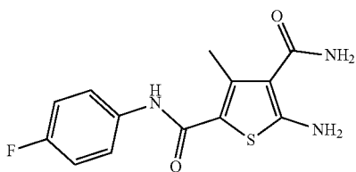
5-Amino-N2-(4-fluorophenyl)-3-methylthiophene-2,4-dicarboxamide (ZW-1037)
