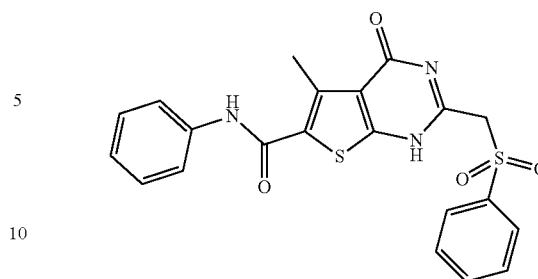
5-Methyl-4-oxo-N-phenyl-2-((phenylsulfonyl)methyl)-1,4-dihydrothieno[2,3-d]pyrimidine-6-carboxamide (ZW-939)
