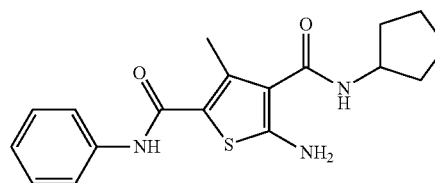
5-Amino-N4-cyclopentyl-3-methyl-N2-phenylthiophene-2,4-dicarboxamide (ZW-895)
