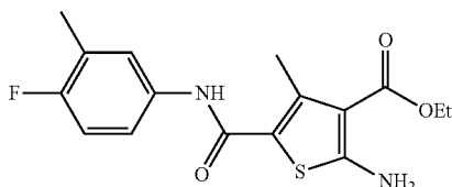
Ethyl 2-amino-5-((4-fluoro-3-methylphenyl)carbamoyl)-4-methylthiophene-3-carboxylate (ZW-1046)
