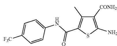
5-Amino-3-methyl-N2-(4-(trifluoromethyl)phenyl)thiophene-2,4-dicarboxamide (ZW-1036)
