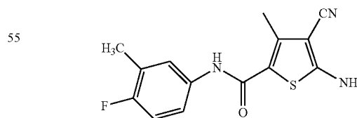
5-Amino-4-cyano-N-(4-fluoro-3-methylphenyl)-3-methylthiophene-2-carboxamide (ZW-1044)
