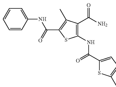
3-Methyl-5-(5-methylthiophene-2-carboxamido)- N2-phenylthiophene-2,4-dicarboxamide (ZW-1056)
