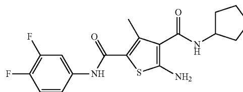
5-Amino-N4-cyclopentyl-N2-(3,4-difluorophenyl)-3-methylthiophene-2,4-dicarboxamide (ZW-894)
