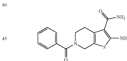
2-Amino-6-benzoyl-4,5,6,7-tetrahydrothieno [2,3-c]pyridine-3-carboxamide (ZW-1072)
