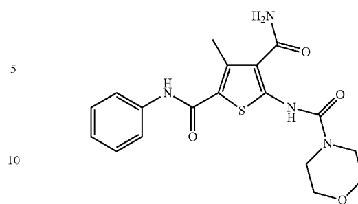
3-methyl-5-(morpholine-4-carboxamido)-N2-phenylthiophene-2,4-dicarboxamide (ZW-1049)
