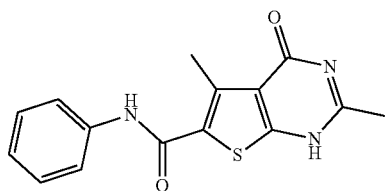
2,5-Dimethyl-4-oxo-N-phenyl-1,4-dihydrothieno[2,3-d]pyrimidine-6-carboxamide (ZW-936)
