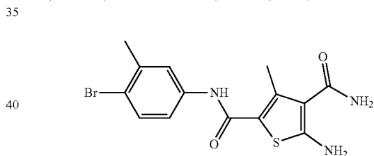
5-Amino-N2-(4-bromo-3-methylphenyl)-3-methylthiophene-2,4-dicarboxamide (ZW-1068)
