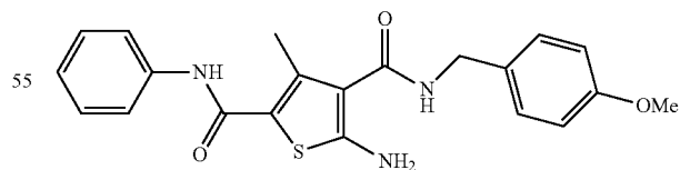
5-Amino-N4-(4-methoxybenzyl)-3-methyl-N2-phenylthiophene-2,4-dicarboxamide (ZW-791)
