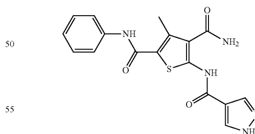
3-Methyl-N2-phenyl-5-(1H-pyrazole-4-carboxamido)thiophene-2,4-dicarboxamide (ZW-1052)
