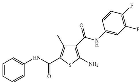
5-Amino-N4-(3,4-difluorophenyl)-3-methyl-N2-phenylthiophene-2,4-dicarboxamide (ZW-933)
