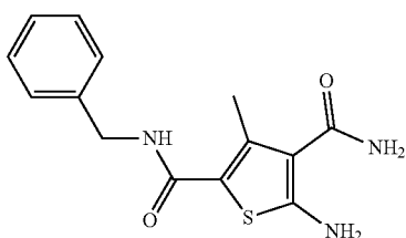
5-Amino-N2-benzyl-3-methylthiophene-2,4-dicarboxamide (ZW-770)
