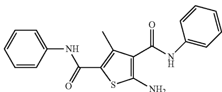
5-Amino-3-methyl-N2,N4-diphenylthiophene-2,4-dicarboxamide (ZW-794)
