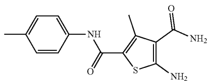
5-Amino-3-methyl-N2-(p-tolyl)thiophene-2,4-dicarboxamide (ZW-771)
