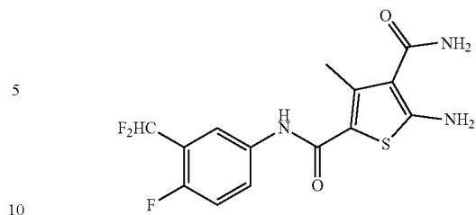
5-Amino-N2-(3-(difluoromethyl)-4-fluorophenyl)-3-methylthiophene-2,4-dicarboxamide (ZW-1066)
