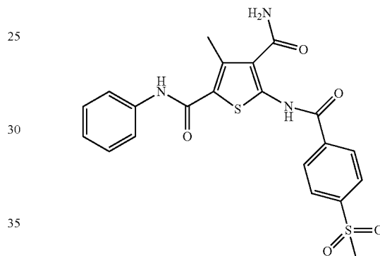
3-Methyl-5-(4-(methylsulfonyl)benzamido)-N2- phenylthiophene-2,4-dicarboxamide (ZW-1073)
