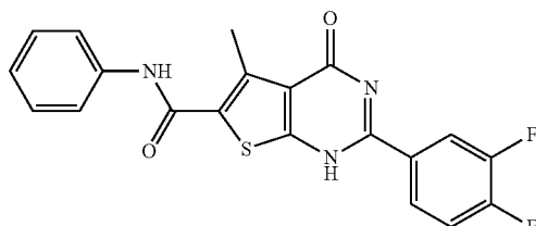
2-(3,4-Difluorophenyl)-5-methyl-4-oxo-N-phenyl-1,4-dihydrothieno[2,3-d]pyrimidine-6-carboxamide (ZW-938)
