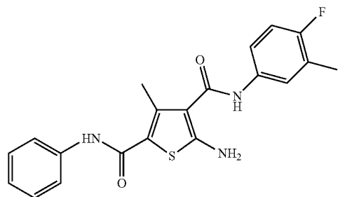
5-Amino-N4-(4-fluoro-3-methylphenyl)-3-methyl-N2-phenylthiophene-2,4-dicarboxamide (ZW-934)
