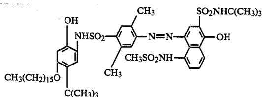
Structural formula B
