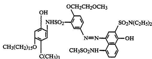
Structural formula B
