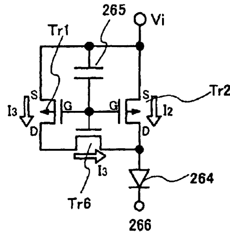
FIG. 25c INVERTED BIAS PERIOD T_i
