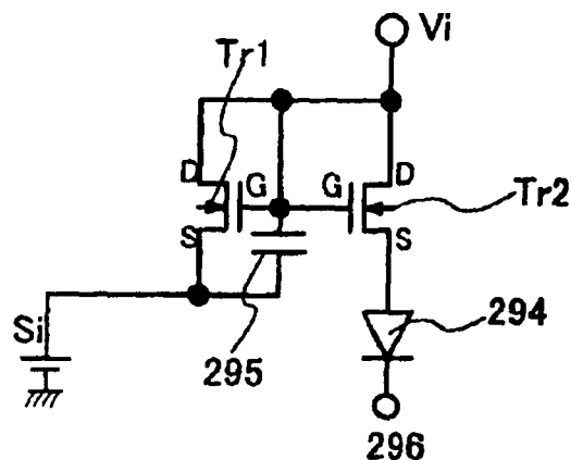
FIG. 31C INVERTED BIAS PERIOD T_i
