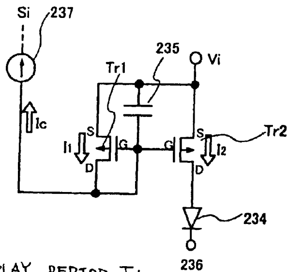
FIG.19A WRITE PERIOD T_a
