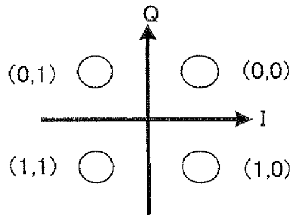
FIG.11A S1(i) SIGNAL POINT ARRANGEMENT
