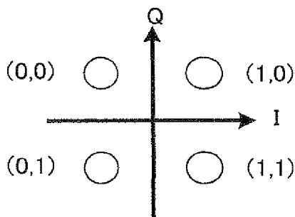
FIG.11B S1(i)' SIGNAL POINT ARRANGEMENT
