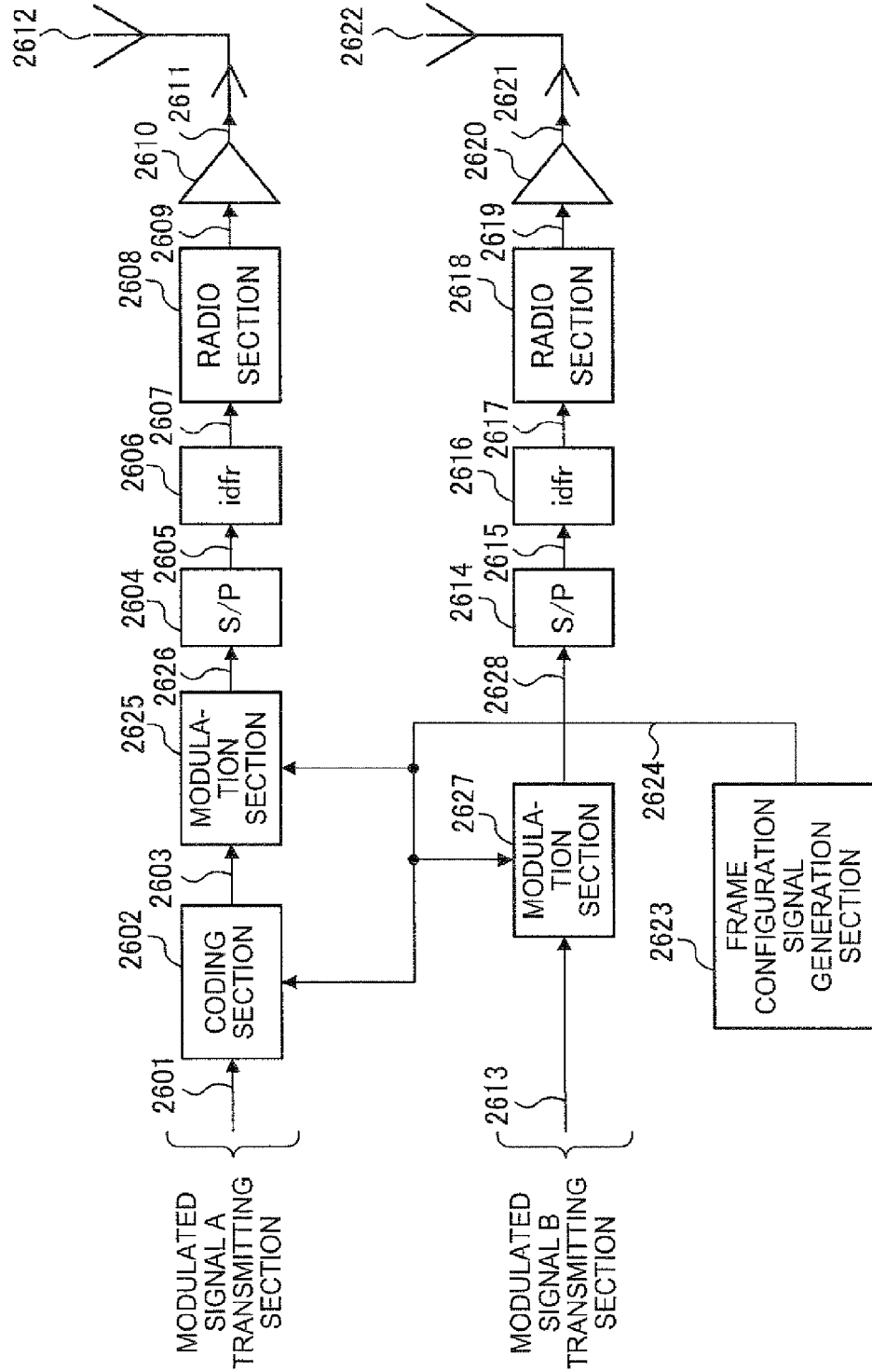
2600 TRANSMITTING APPARATUS
