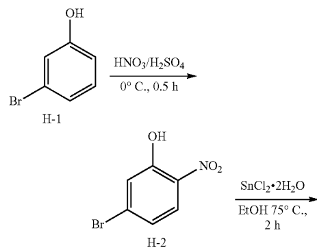
Reaction Scheme H
