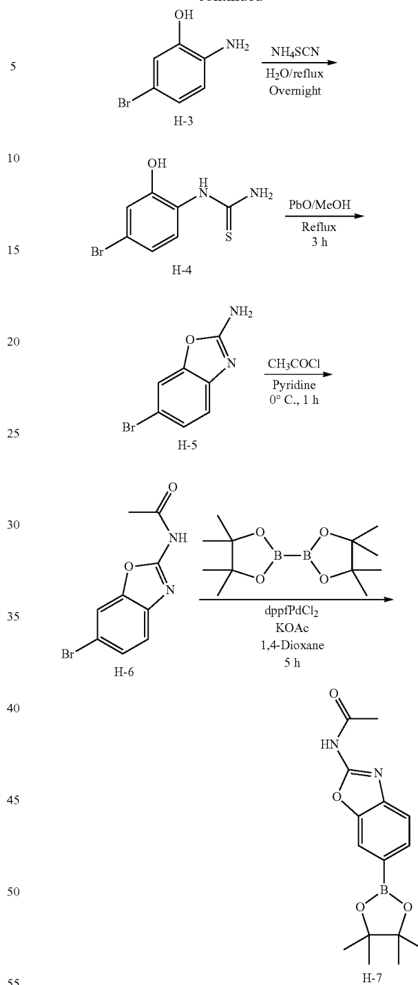
Reaction Scheme I
