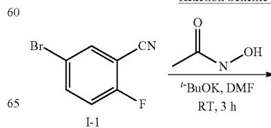
Reaction Scheme I
