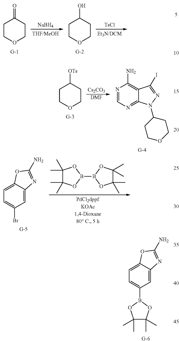
Reaction Scheme G
