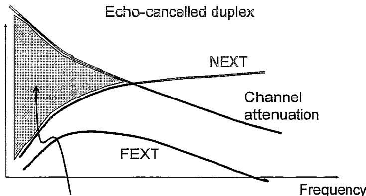
Available SNR in both downstream and upstream direction - full time
