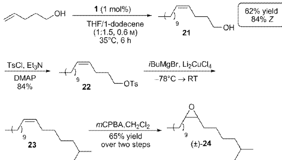
Scheme 6. Synthesis of pheromone (±)-24. DMAP = 4-dimethylamino-pyridine, m CPBA = meta -chloroperbenzoic acid, Ts = 4-toluenesulfonyl.
