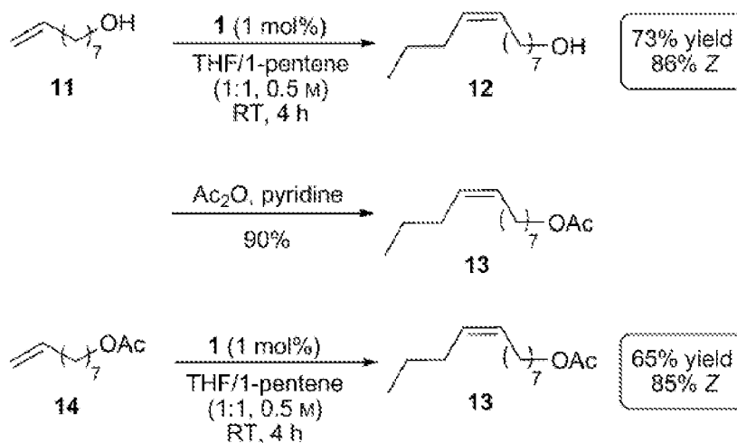
[0166] Scheme 3. Syntheses of pheromones 12 and 13 .
