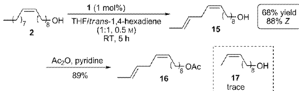
[0167] Scheme 4. Synthesis of pheromone 16 .
