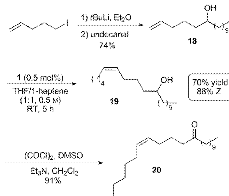
[0168] Scheme 5. Synthesis of pheromone 20.
