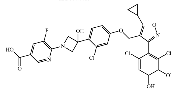
M1 m/z 638.0664 Abundance by UV 23%
