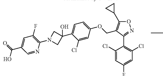
Example 3 m/z 622.0512
