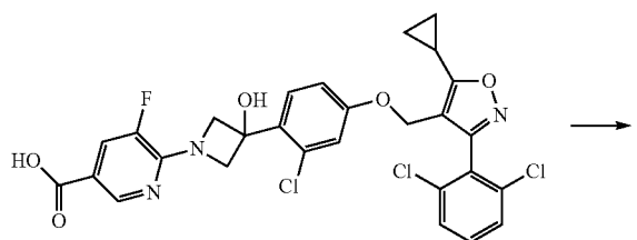
Comparative Example 1 m/z 604.0610
