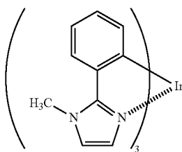
[Chemical formula 4]
