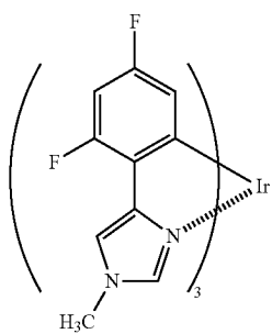
[Chemical formula 7]
