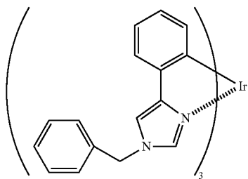
[Chemical formula 7]
