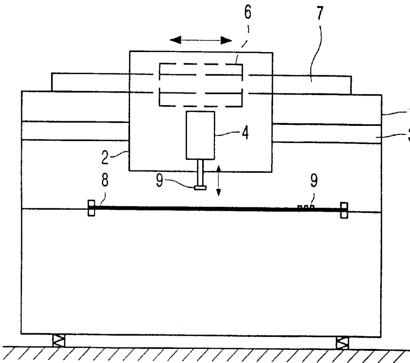
FIG. 6 PRIOR ART
