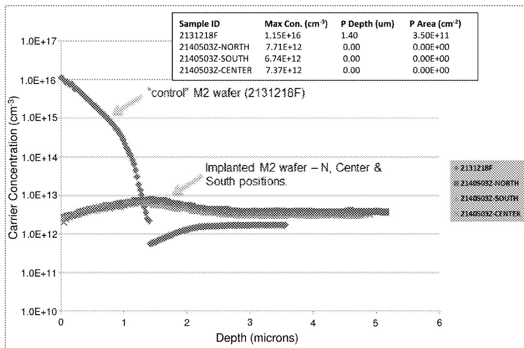
Carrier Concentration vs. Depth
