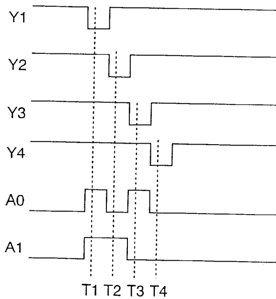
FIG. 2 (PRIOR ART)
