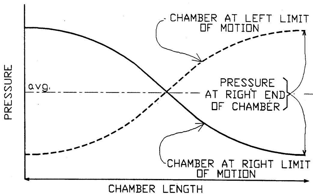
DIAGRAM: PRESSURE DISTRIBUTION ALONG CHAMBER
