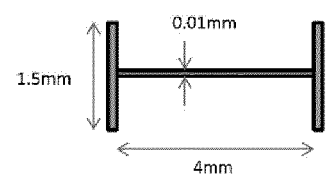
SHAPE OF RESIN FOR FIXING
