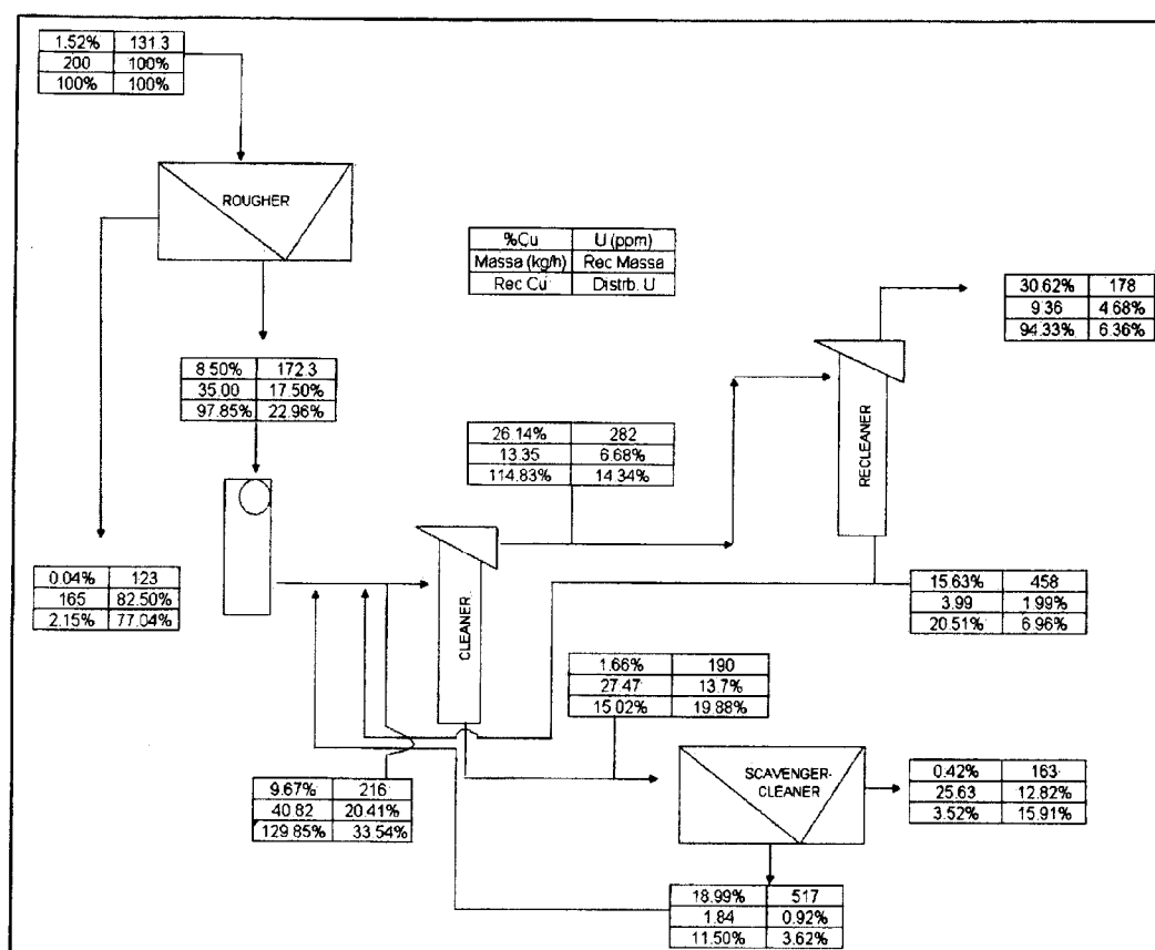
Figure 3 - Flotation flowchart of the run 2
