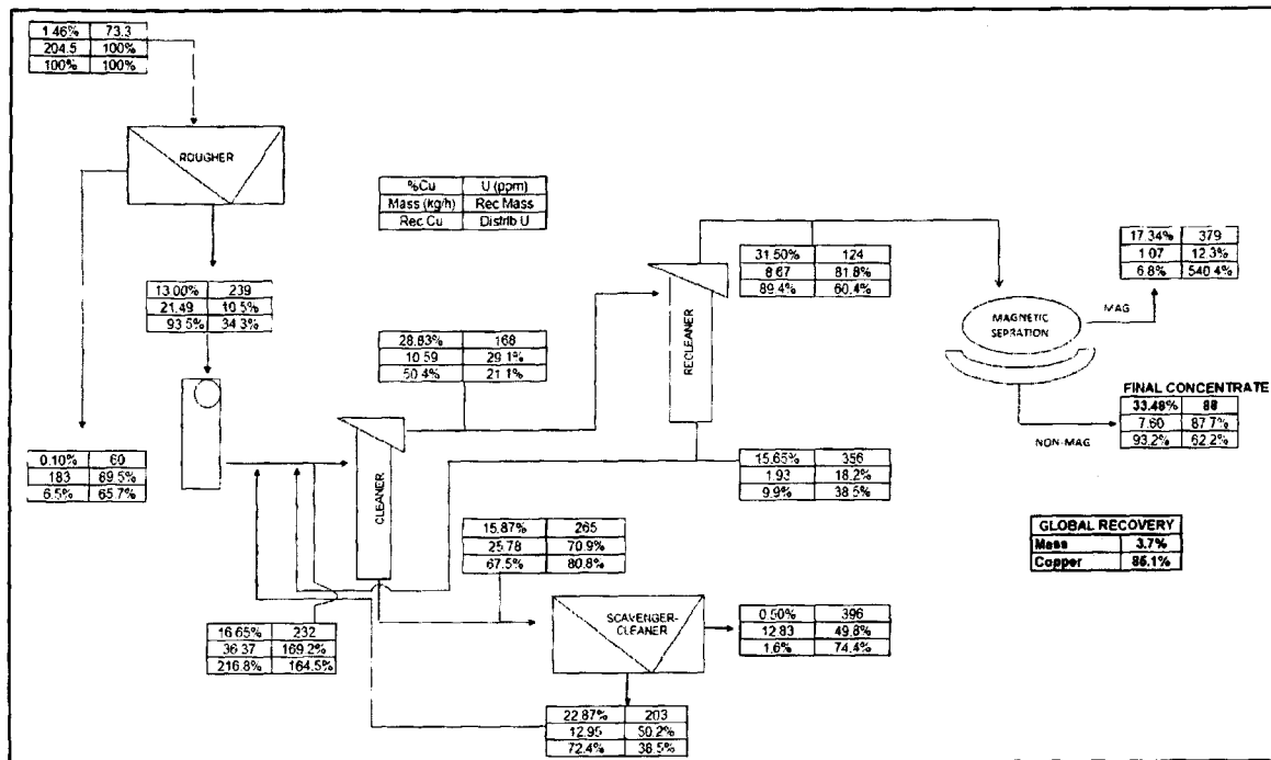
Figure 14 - 3 rd plant campaign.
