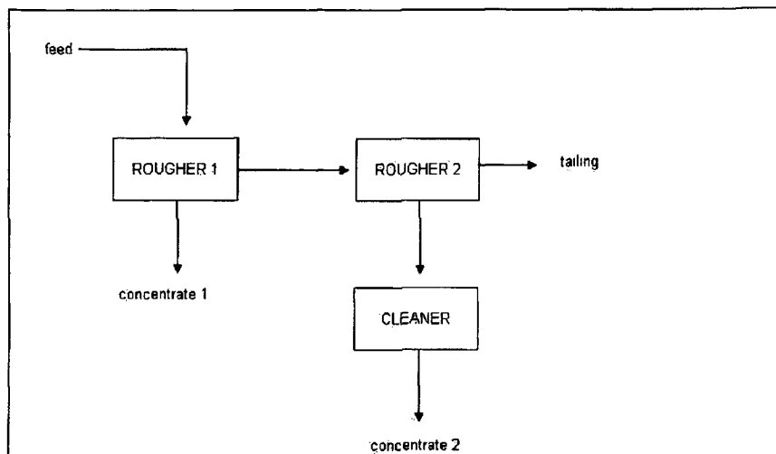
Fine flotation of the cleaner flotation circulating load
