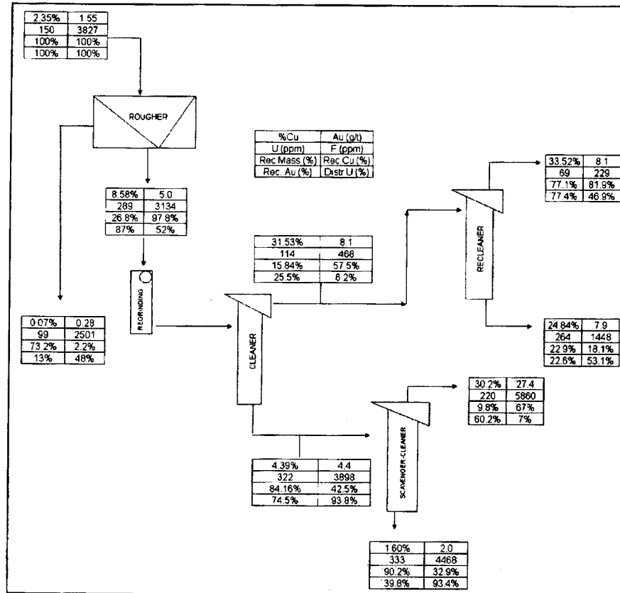
Figure 7 - Flotation flowchart of runs 1 and 2.
