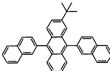
[Chemical Formula 27]
