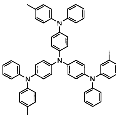
[Chemical Formula 13]
