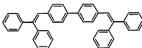
[Chemical Formula 22]
