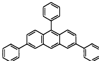
[Chemical Formula 28]
