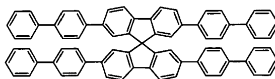
[Chemical Formula 23]
