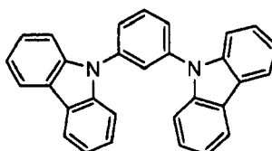
[Chemical Formula 26]
