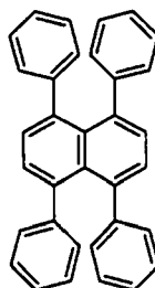
[Chemical Formula 29]
