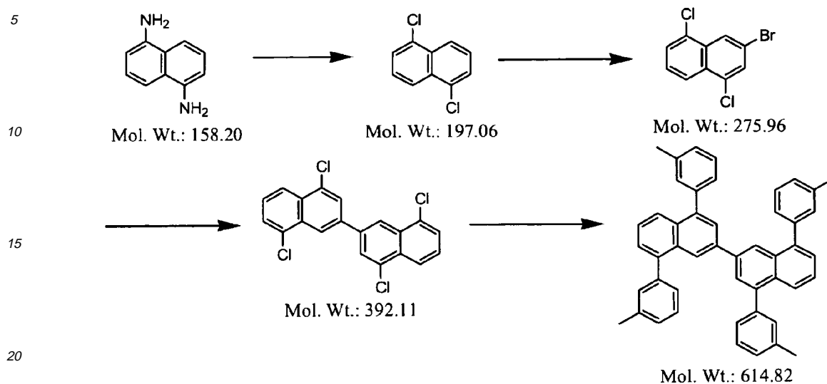
[Chemical Formula 34]
