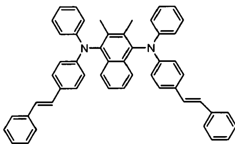
[Chemical Formula 14]
