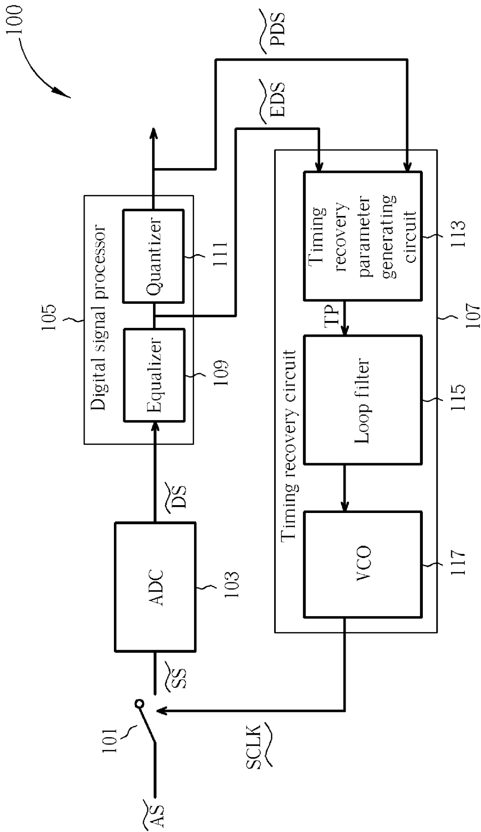
FIG. 1 PRIOR ART
