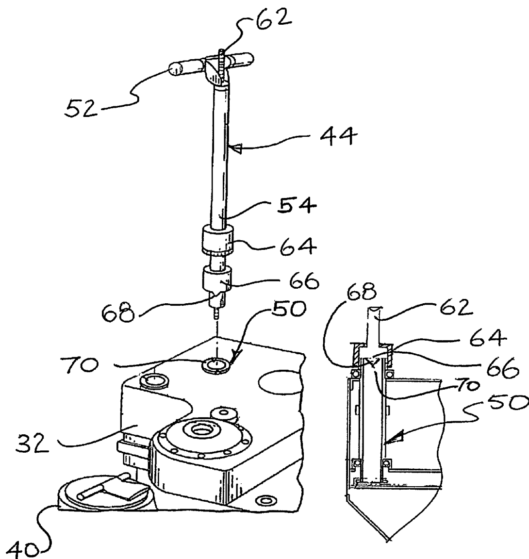
FIG. 2 PRIOR ART
