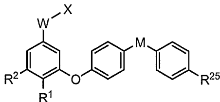
Formula Ih
