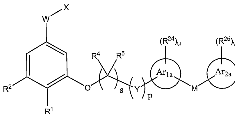
Formula Ia
