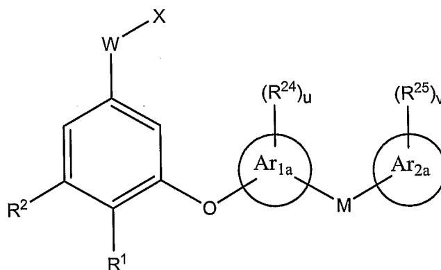
Formula Id
