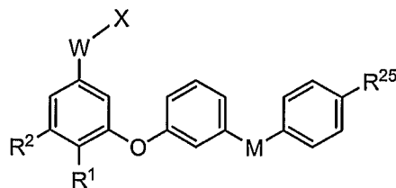
Formula If
