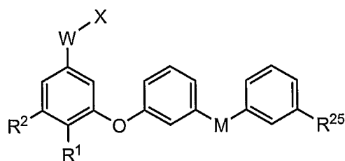
Formula Ie
