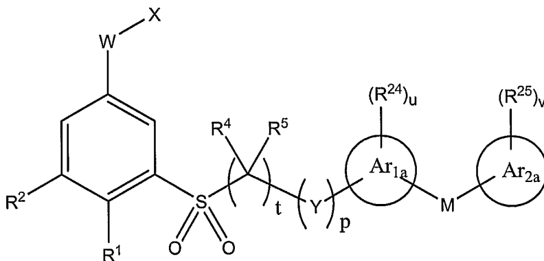
Formula Ib
