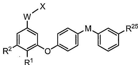
Formula Ig
