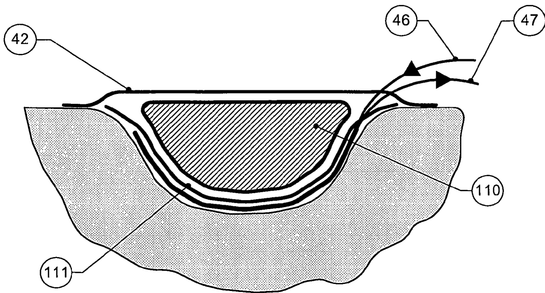
Section Through X-X
