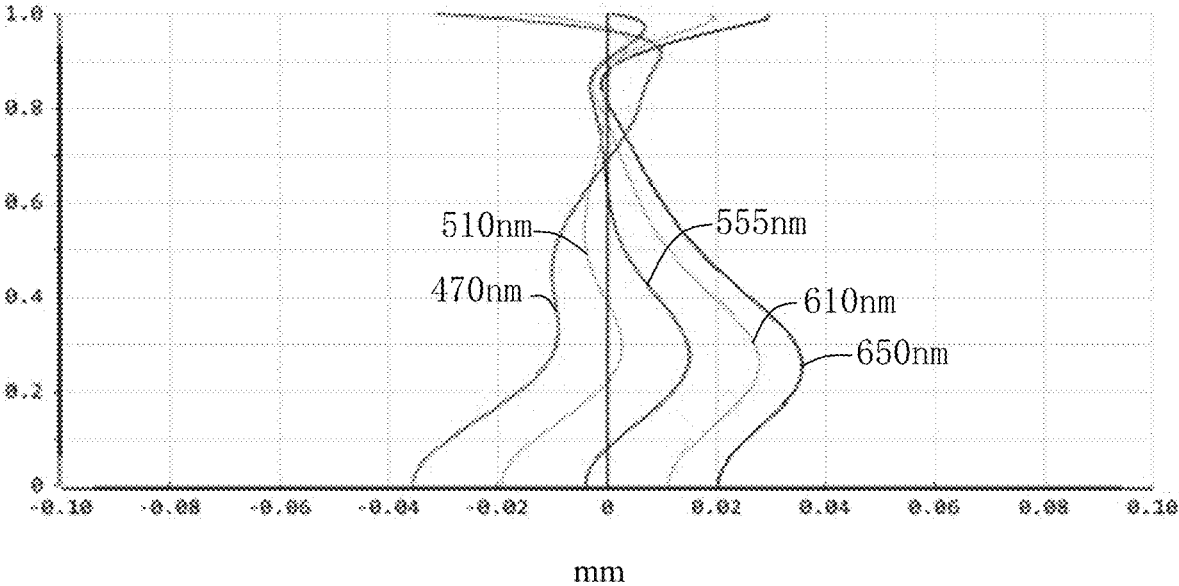
axial chromatic aberration
