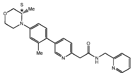
(Compound 119)
