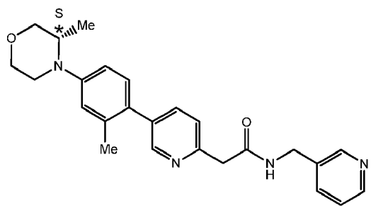
(Compound 118)
