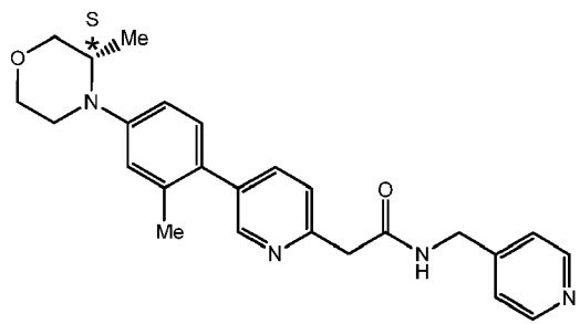
(Compound 117)
