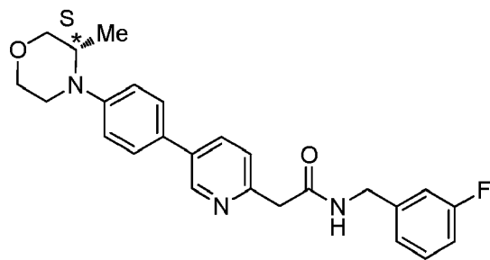
(Compound 102)
