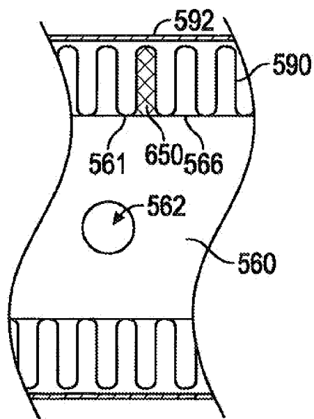
FIG. 12C (Section H-H)
