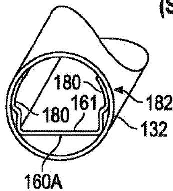
FIG. 6C (Section C-C)
