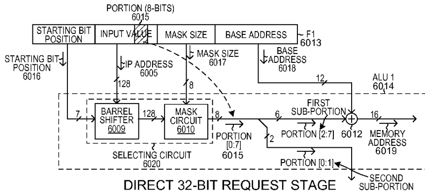
DIRECT 32-BIT MEMORY PACKING SCHEME FIG. 40
