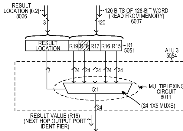
DIRECT 24-BIT LOOK-UP STAGE FIG. 49
