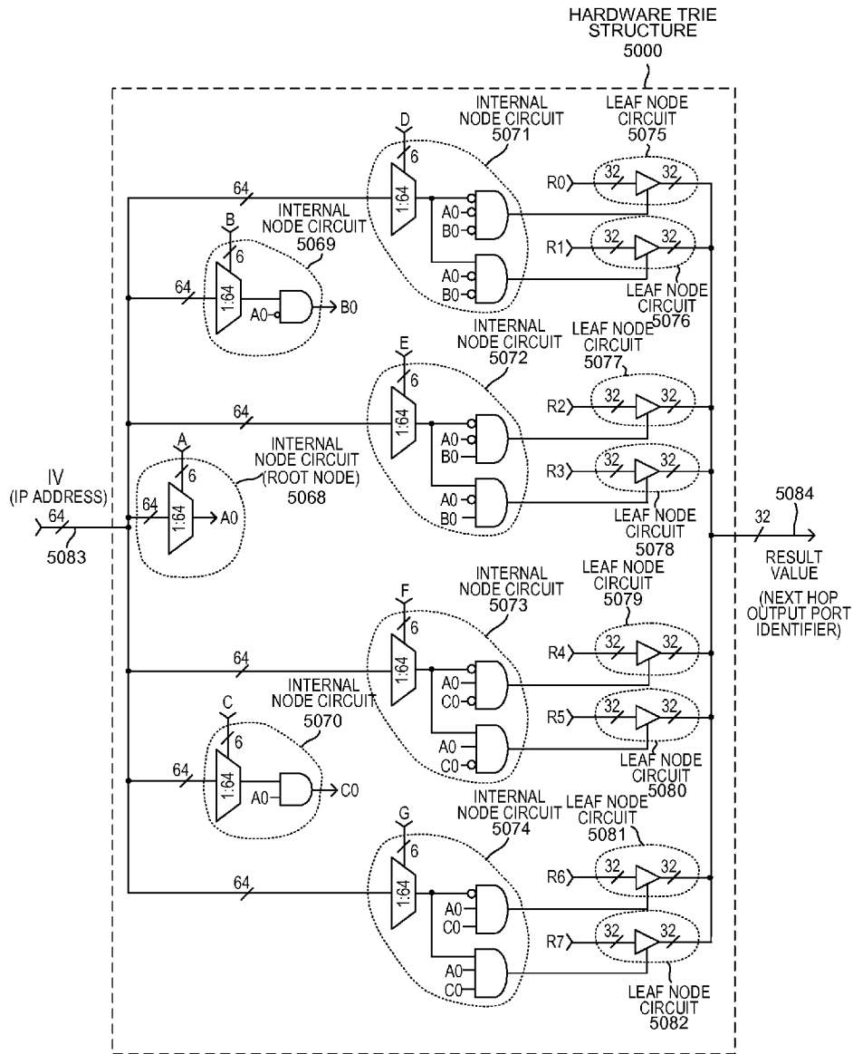
HARDWARE TRIE STRUCTURE
