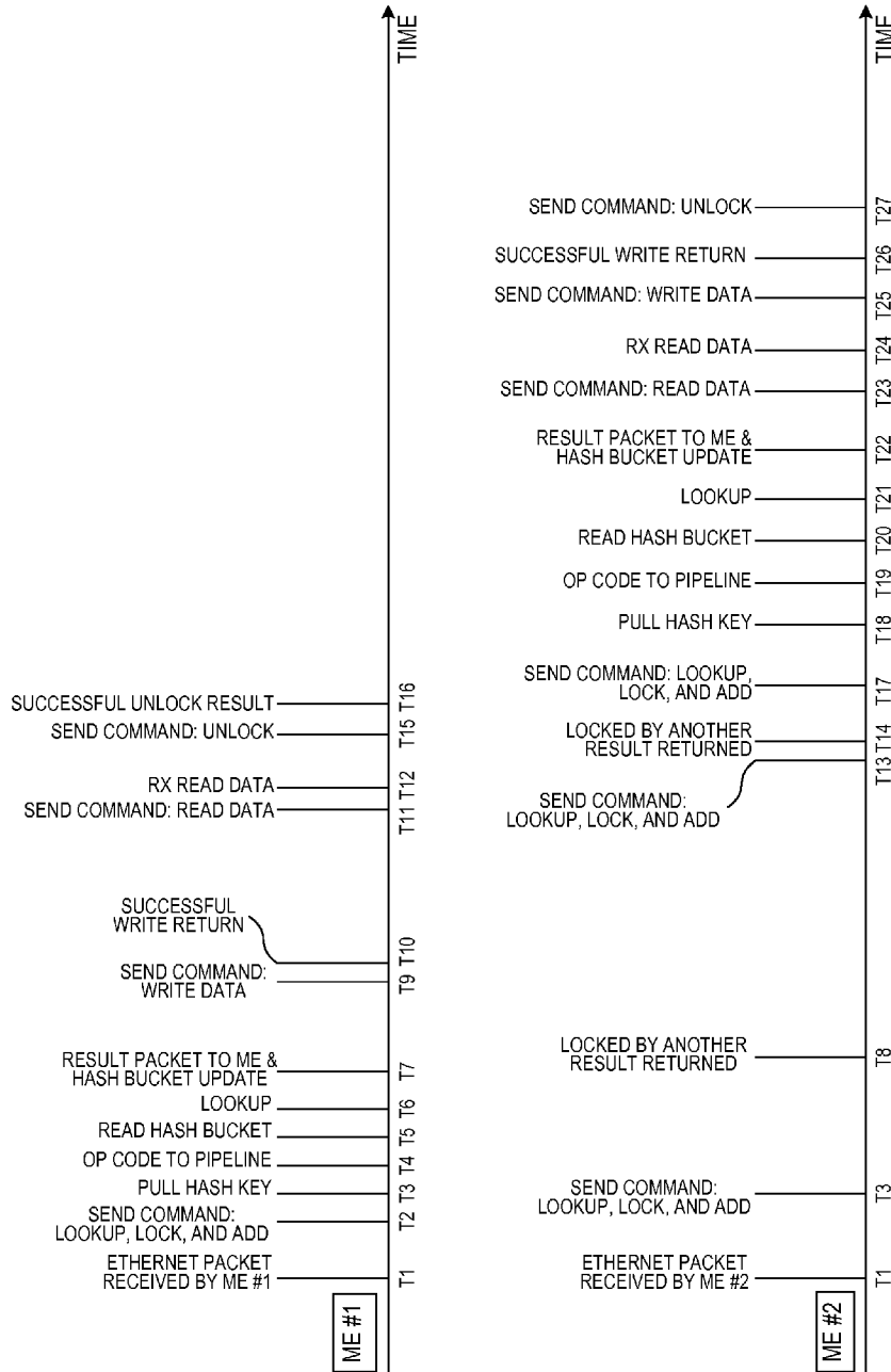
LOOKUP, LOCK, AND ADD TIMING DIAGRAM FIG. 14
