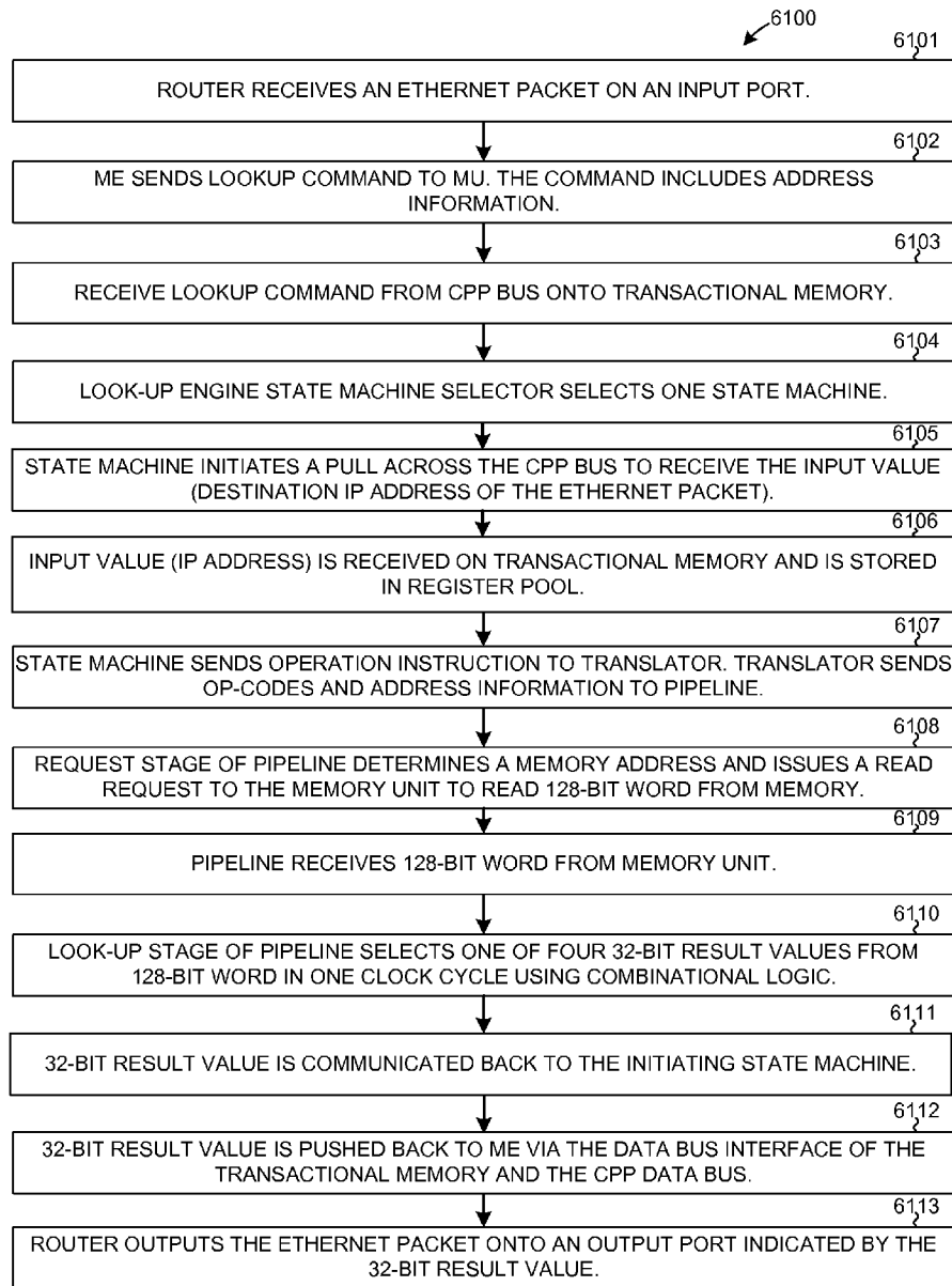
DIRECT 32-BIT LOOKUP FLOWCHART FIG. 44
