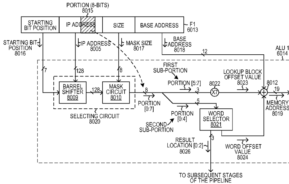
DIRECT 24-BIT REQUEST STAGE FIG. 48
