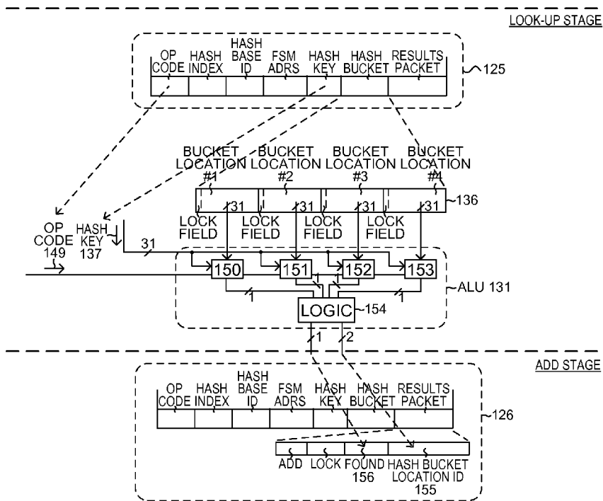
LOOK-UP STAGE FIG. 20
