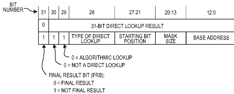
DIRECT RESULT VALUE FIG. 43
