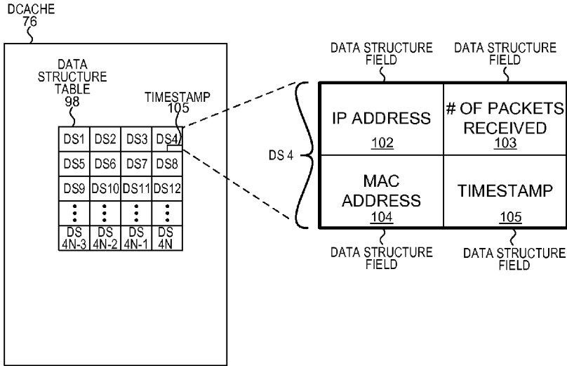
DATA STRUCTURE DIAGRAM FIG. 13
