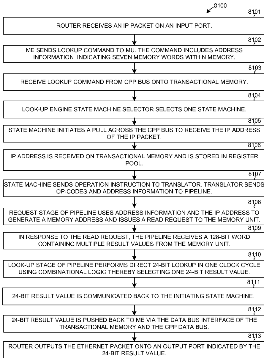
DIRECT 24-BIT LOOK-UP FLOWCHART FIG. 50
