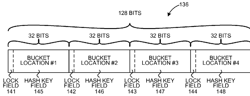
HASH BUCKET FIG. 19
