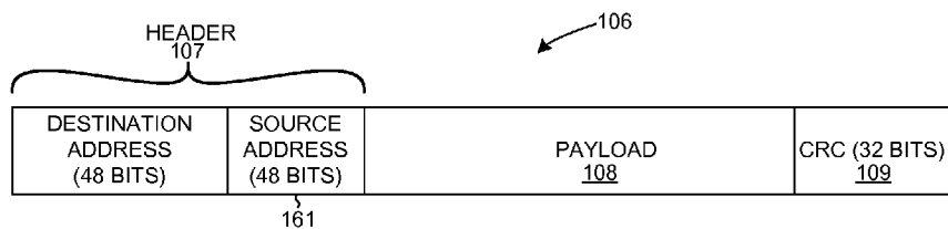
ETHERNET PACKET FIG. 15
