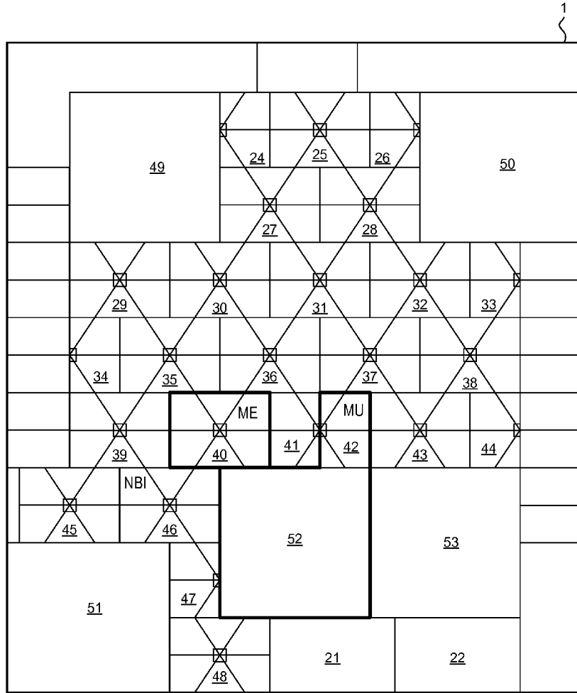
COMMAND-PUSH-PULL (CPP) DATA BUS STRUCTURE
