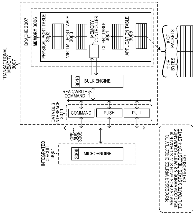
TRANSACTIONAL MEMORY PERFORMING COUNT UPDATE (PRIOR ART)
