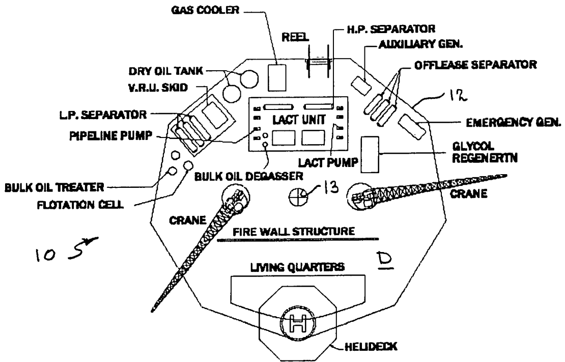
MAIN-DECK EQUIPMENT LAYOUT
