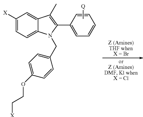
Scheme 13
