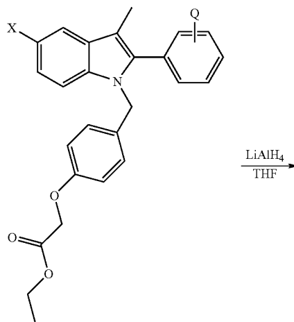
Scheme 10
