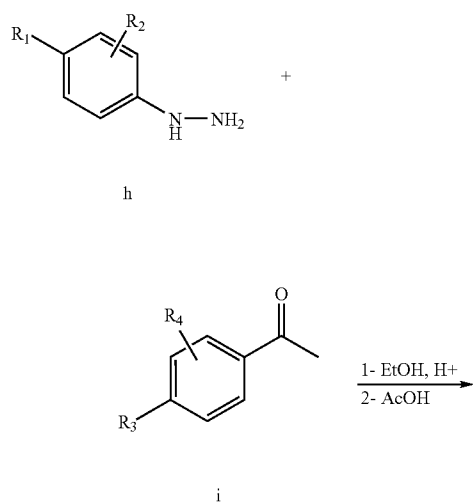
Scheme 2
