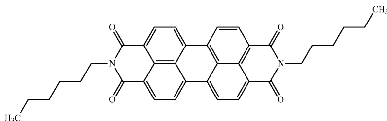
HexPTC
