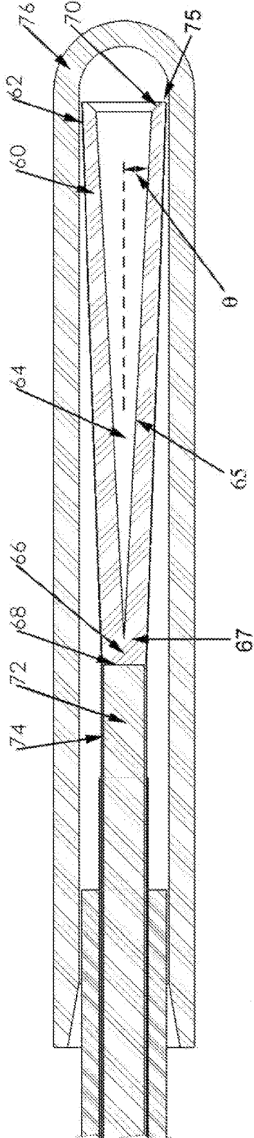
FIG. 9 (Prior Art, '097)
