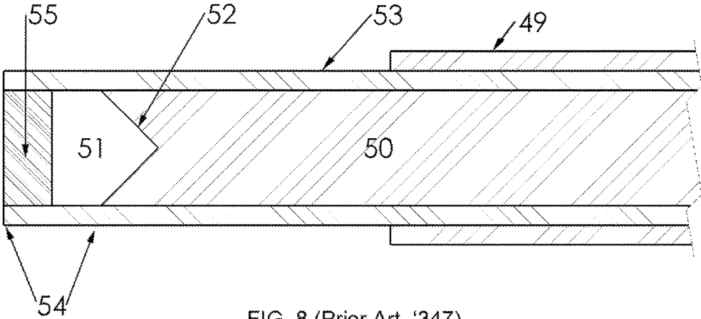
FIG. 8 (Prior Art, '347)
