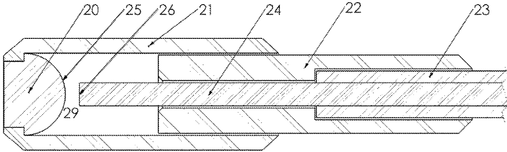
FIG. 3 (Prior Art, '684)
