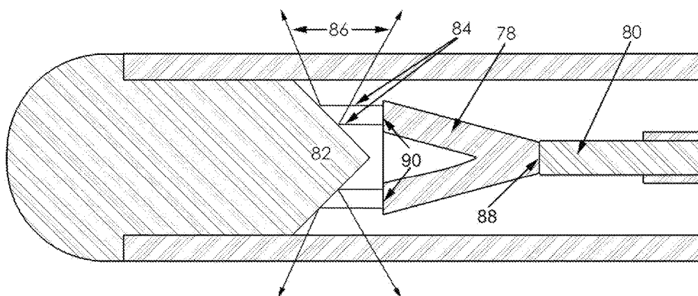
FIG. 10 (Prior Art, '438)
