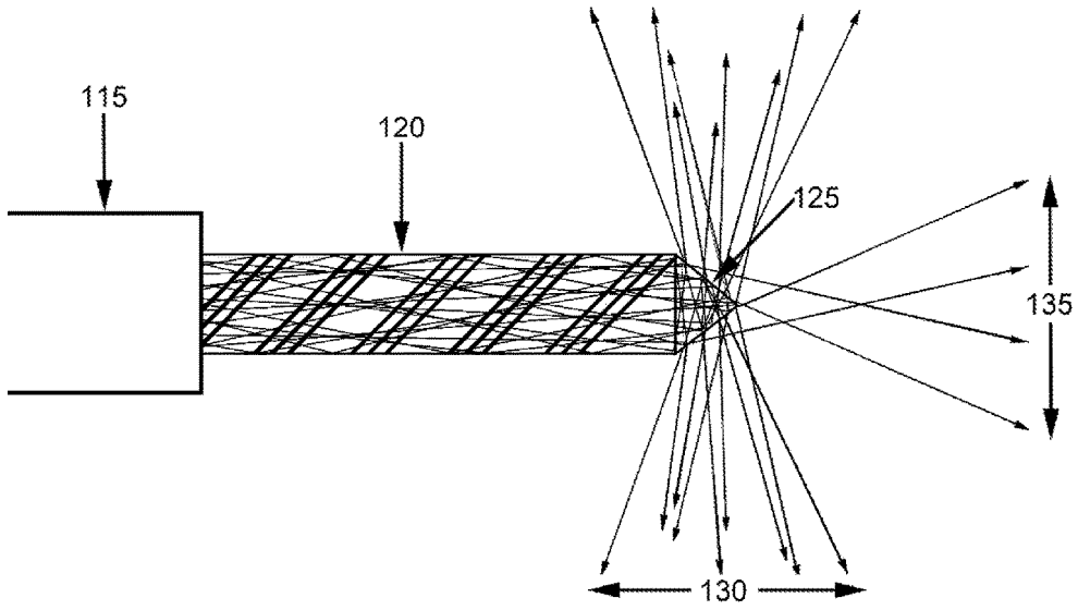
FIG. 12 (Prior Art)
