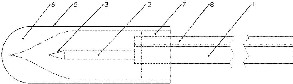
FIG. 1 (Prior Art, '390)
