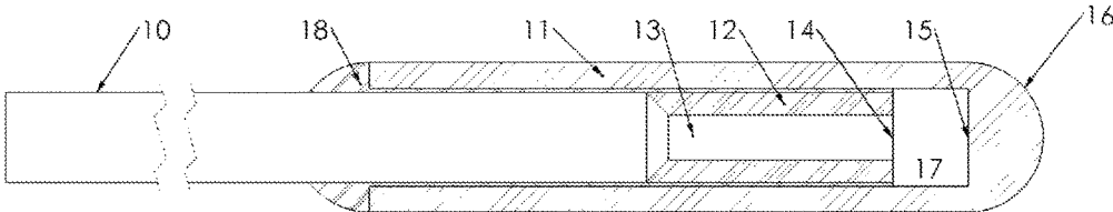
FIG. 2 (Prior Art, '877)
