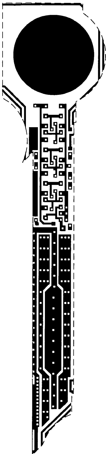
Metal 1 mask
