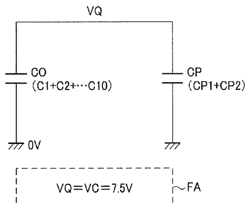
FIG. 5B MAXIMUM DATA VOLTAGE
