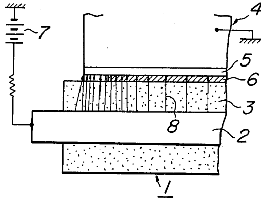
FIG. 2 PRIOR ART
