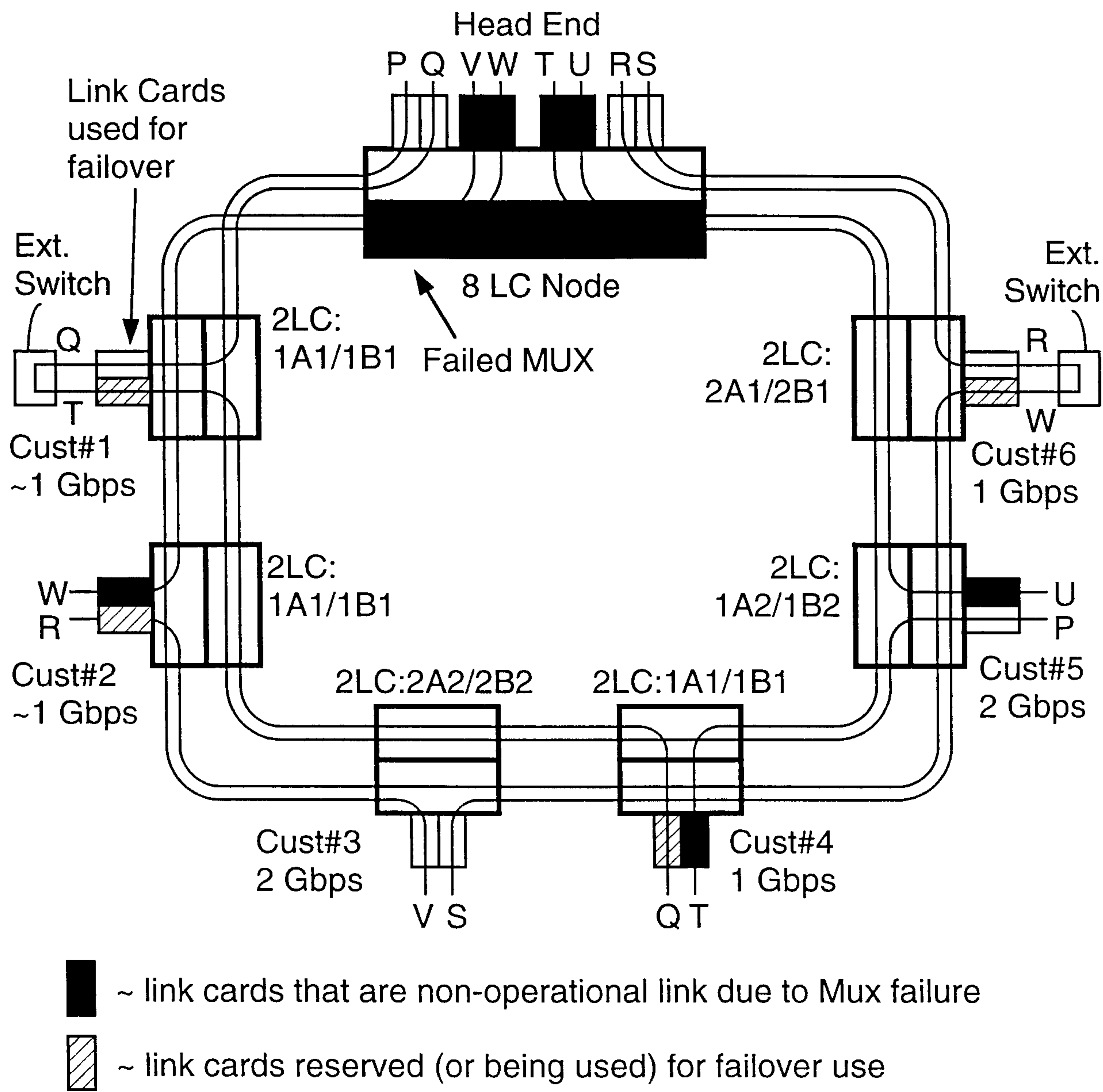
Failed Head End MUX Failover
