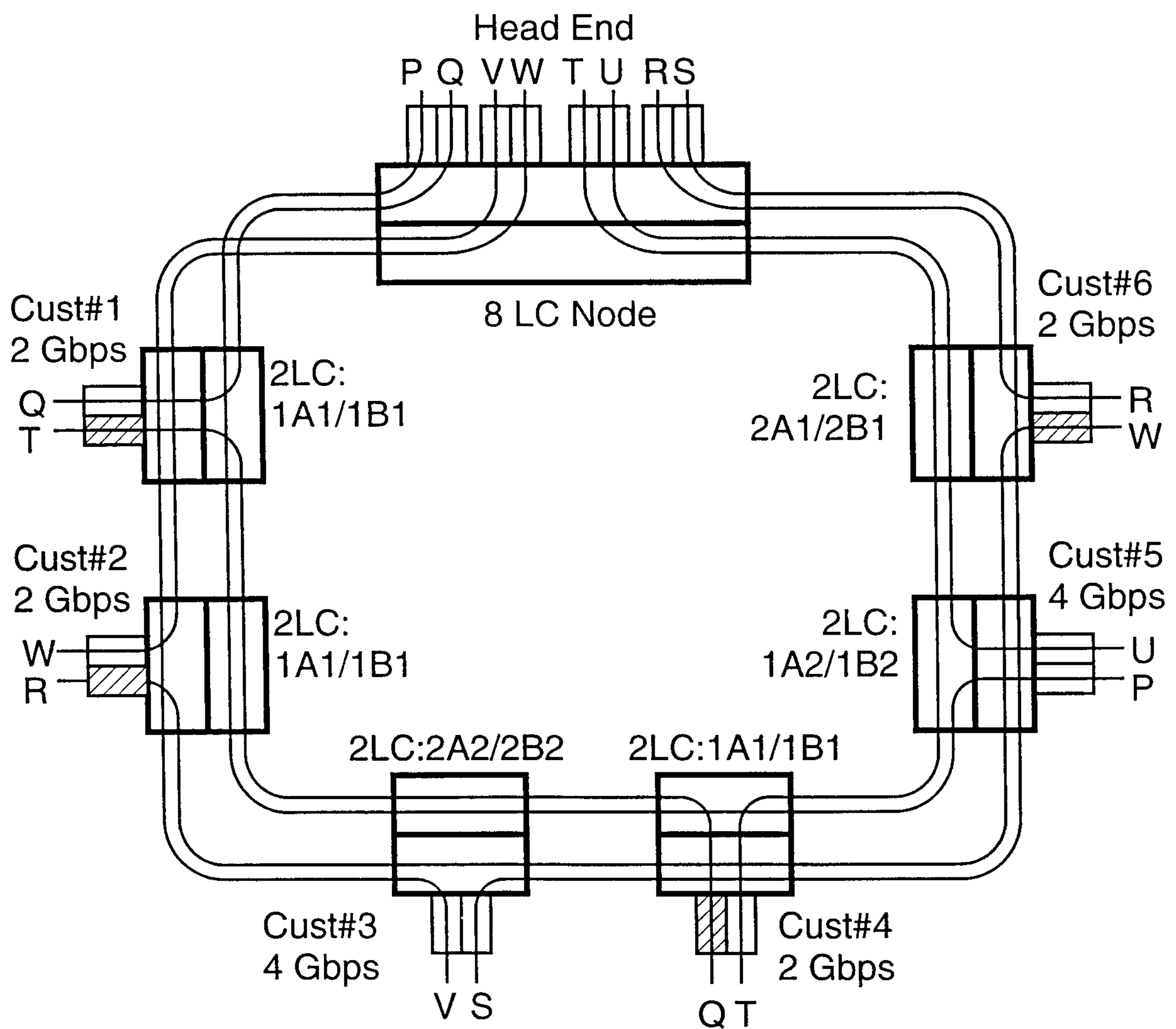
Exemplary Optical Communication System Deployment
