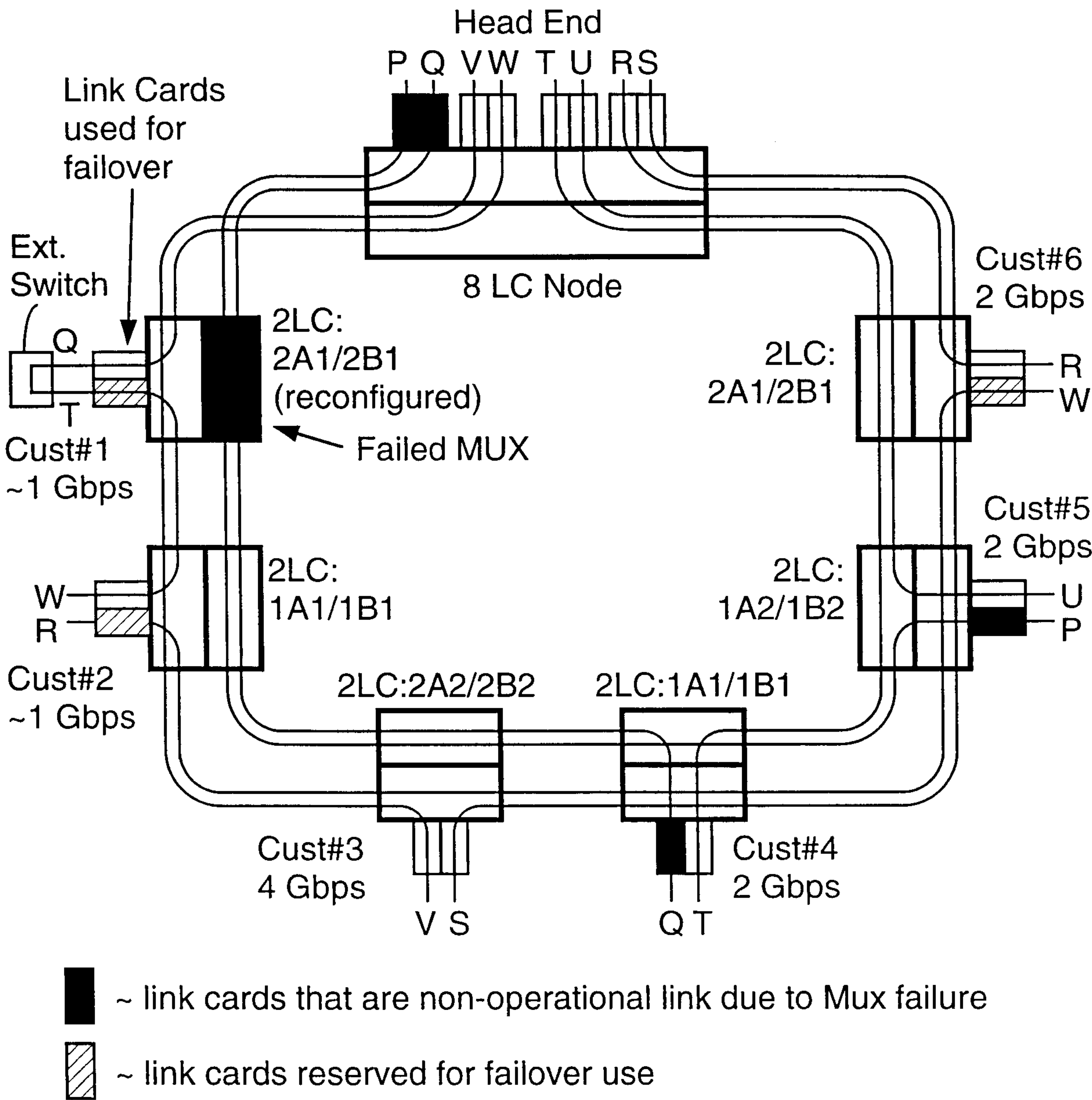
Failed Customer MUX Failover
