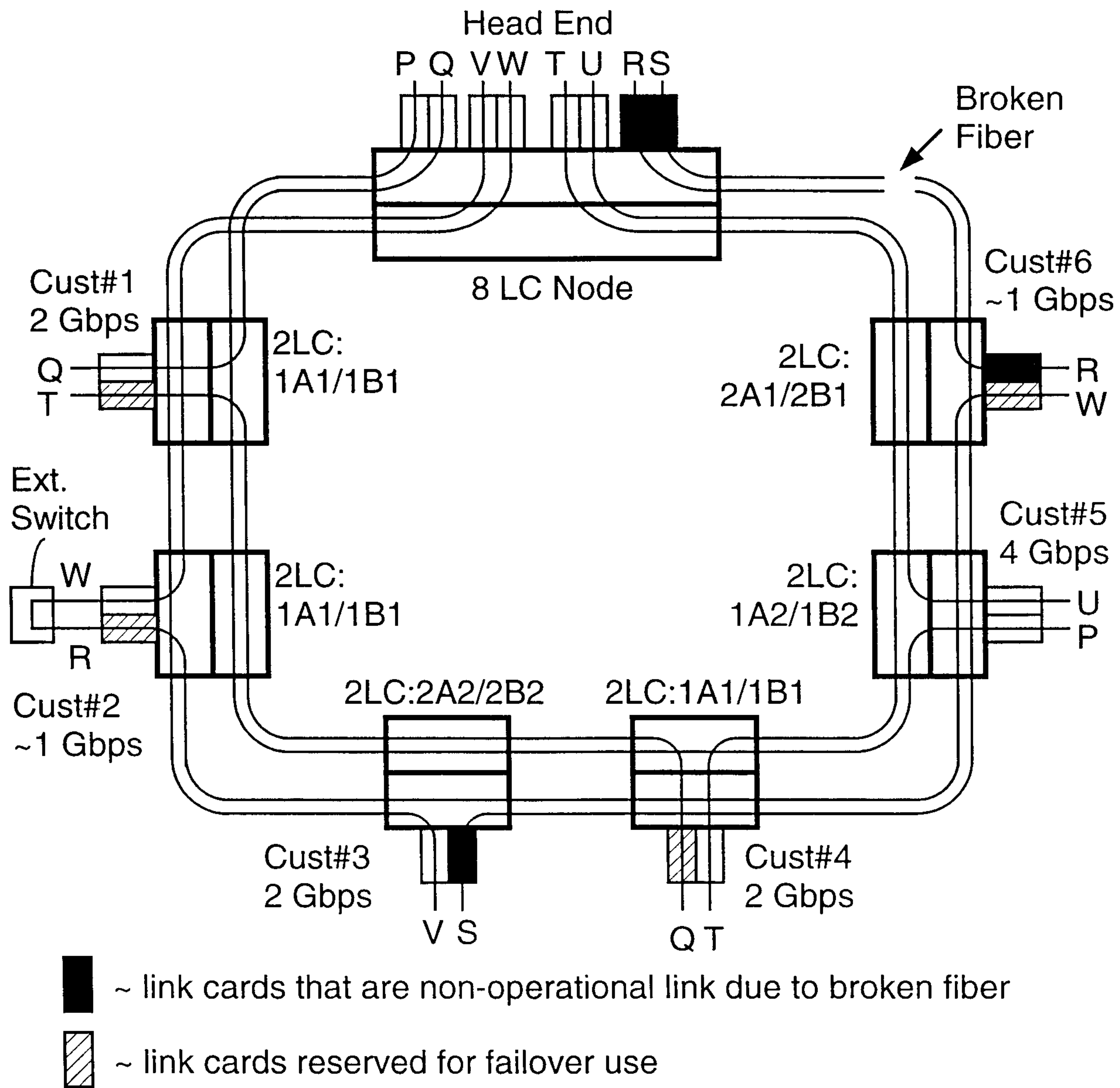
Broken Fiber Failover
