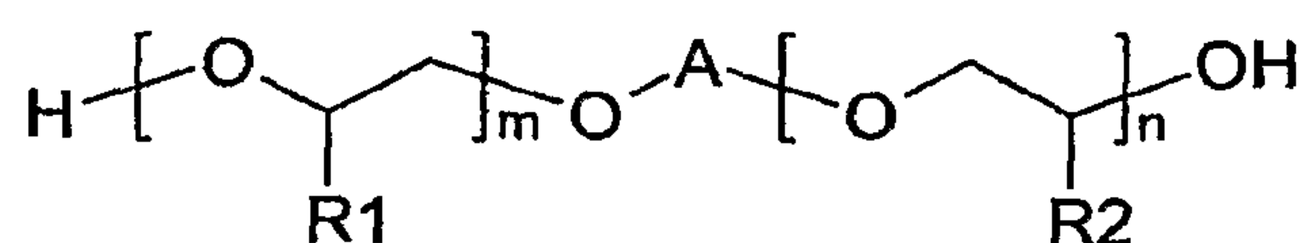
Formula (I')
