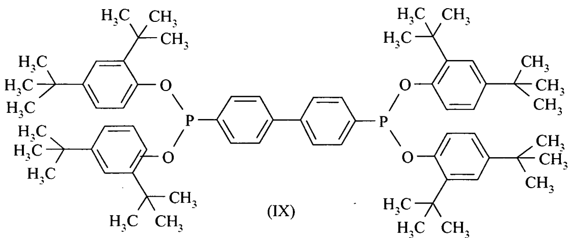
Tetrakis(2,4-di-tert-butylphenyl)[1,1-biphenyl]- 4,4'diylbisphosphonite
