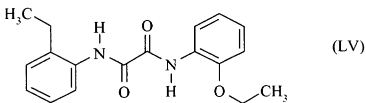
2-Ethyl,- 2'-ethoxy-oxalanilide
