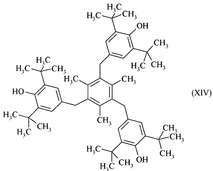
1,3,5-Trimethyl-2,4,6-tris(3,5-di-tert-butyl-4-hydroxybenzyl)benzene
