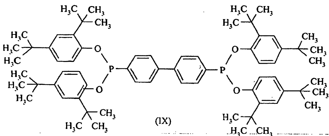
Tetrakis(2,4-di-tert.-butylphenyl)[1,1-biphenyl]-4,4'-diylbisphosphonit
