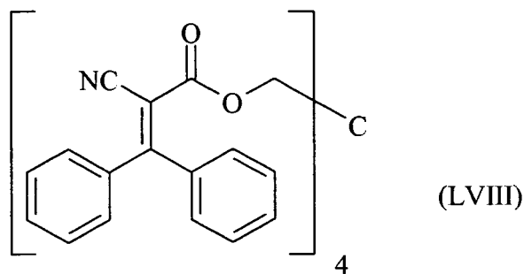
1,3-bis-[(2'-cyano-3',3'-diphenylacryloyl)oxy]-2,2-bis-{[(2'-cyano-3',3'-diphenylacryloyl)oxy]methyl}-propane
