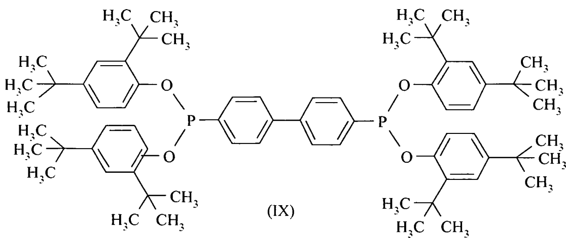
Tetrakis(2,4-di-tert-butylphenyl)[1,1'-biphenyl]-4,4'-diylbisphosphite
