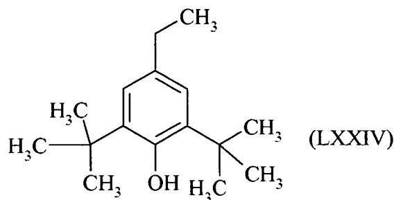
2,6-Di-tert.-butyl-4-ethyl-phenol
