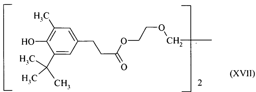
Triethyleneglycolbis-3-(3-tert-butyl-4-hydroxy-5-methylphenyl)-propionate
