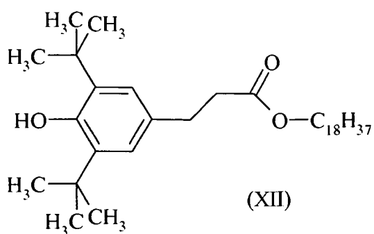
Octadecyl 3,5-di-tert-butyl-4-hydroxyhydrocinnamate
