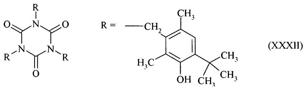
1,3,5-Tris(4-tert-butyl-3-hydroxy-2,6-dimethylbenzyl)-1,3,5-triazine-2,4,6-(1H,3H,5H)-trione
