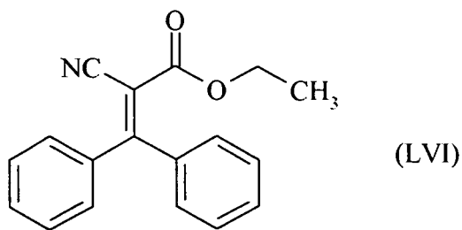
Ethyl-2-cyano-3,3-diphenylacrylate
