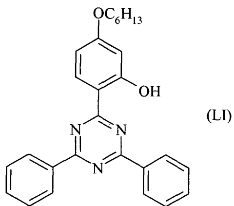
-(4,6-diphenyl-1,3,5-triazin-2-yl)-5-[(hexyl)oxy]-phenol
