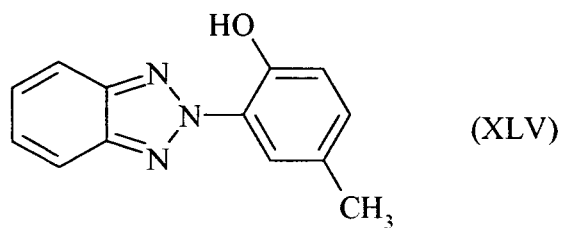
2-(2'-hydroxy-5'-methylphenyl)benzotriazole
