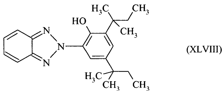
2-(2'-Hydroxy-3',5'-ditert-butylphenyl)-benzotriazole
