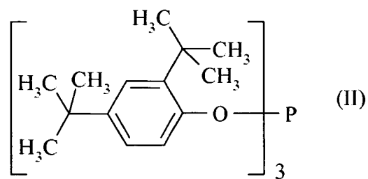
Tris(2,4-di-tert-butylphenyl)phosphite
