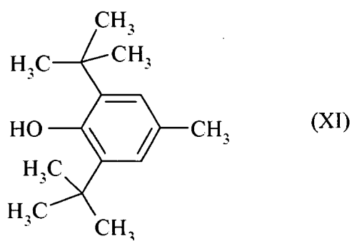
2,6-Di-tert.-butyl-4-methyl-phenol
