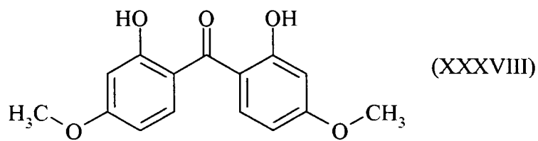
bis-(2-hydroxy-4-methoxyphenyl)methanone
