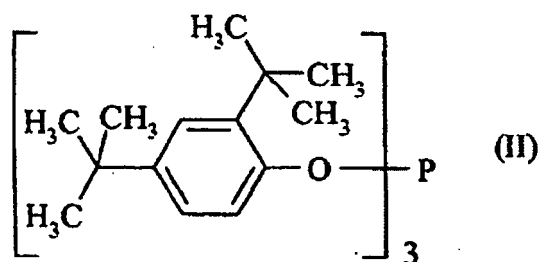
Tris(2,4-di-tert.-butylphenyl)phosphit
