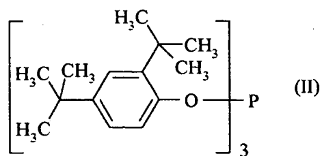
tris(2,4-di-tert-butylphényl)phosphite
