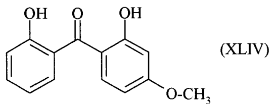
2,2'-Dihydroxy-4-methoxybenzophenone
