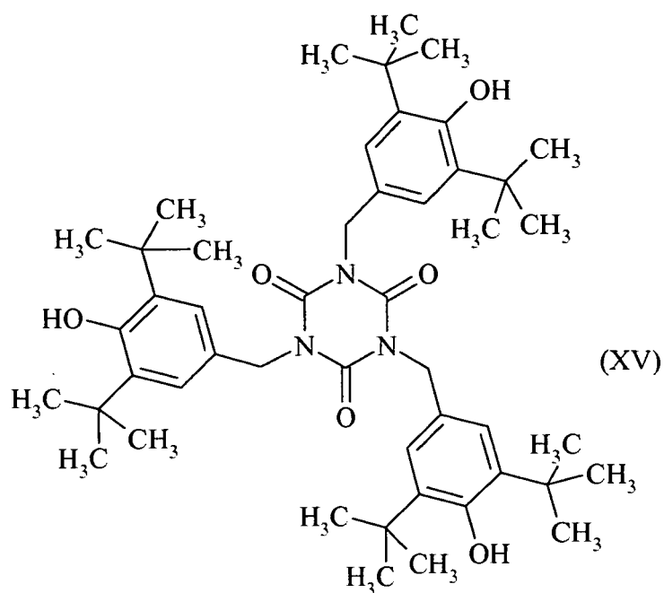
1,3,5-Tris(3,5-di-tert-butyl-4-hydroxybenzyl)isocyanurate
