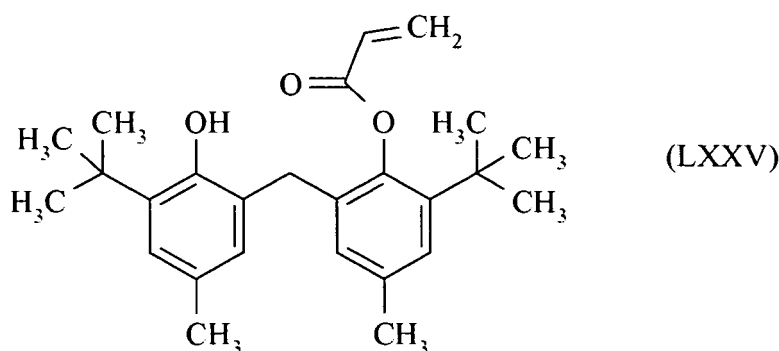
2-(1,1-dimethylethyl)-6-[3-(1,1-dimethylethyl)-2-hydroxy-5-methylphenyl]-4-methylphenyl-acrylate
