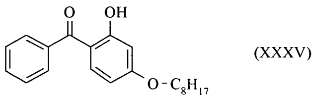
2-Hydroxy-4-n-octyloxybenzophenone
