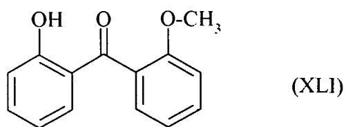
2-Hydroxy-2'-methoxybenzophenone
