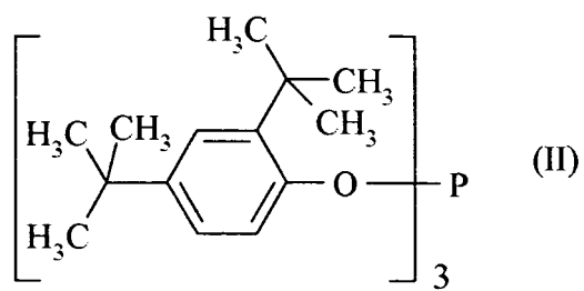
Tris(2,4-di-tert-butylphenyl)phosphite
