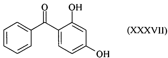
2,4-Dihydroxybenzophenone
