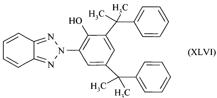
2-[2-Hydroxy-3,5-di-(a,a-dimethylbenzyl)phenyl]-2H-benzotriazole
