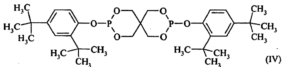
Bis(2,4-di-t-butylphenyl)pentaerythritdiphosphit
