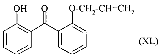
2-Hydroxy-2'-allyloxybenzophenone
