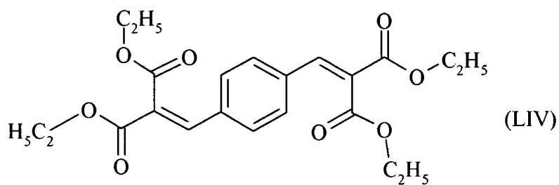
Tetra-ethyl-2,2'-(1,4-phenylene-dimethyldene)-bismalonate
