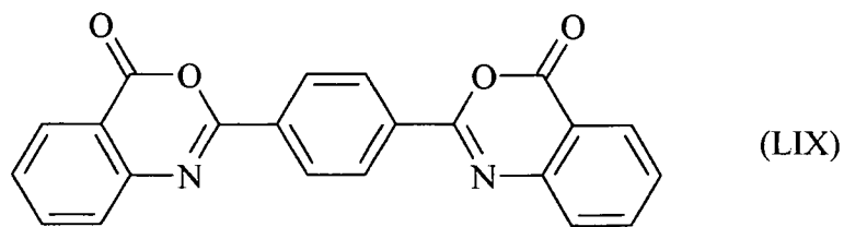
2,2'-(1,4-Phenylene)bis[4H-3,1-benzoxazin-4-one]
