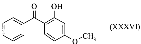
2-Hydroxy-4-methoxybenzophenone
