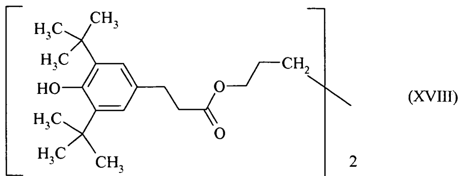
1,6-Hexanediolbis-3-(3,5-di-tert-butyl-4-hydroxyphenyl)propionate
