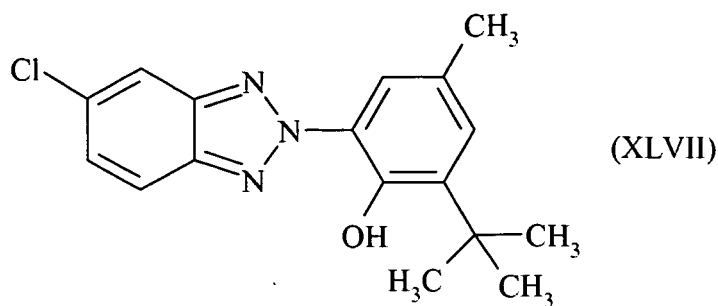
2-(5-chlorobenzotriazol-2-yl)-4-methyl-6-tert-butyl-phenol
