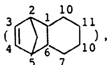
10-methyltricyclo[4,4,0,12,5]-3-undecene, pentacyclo[6,5,1,13,6,02,7,09,13]-4,10-pentadecadiene
