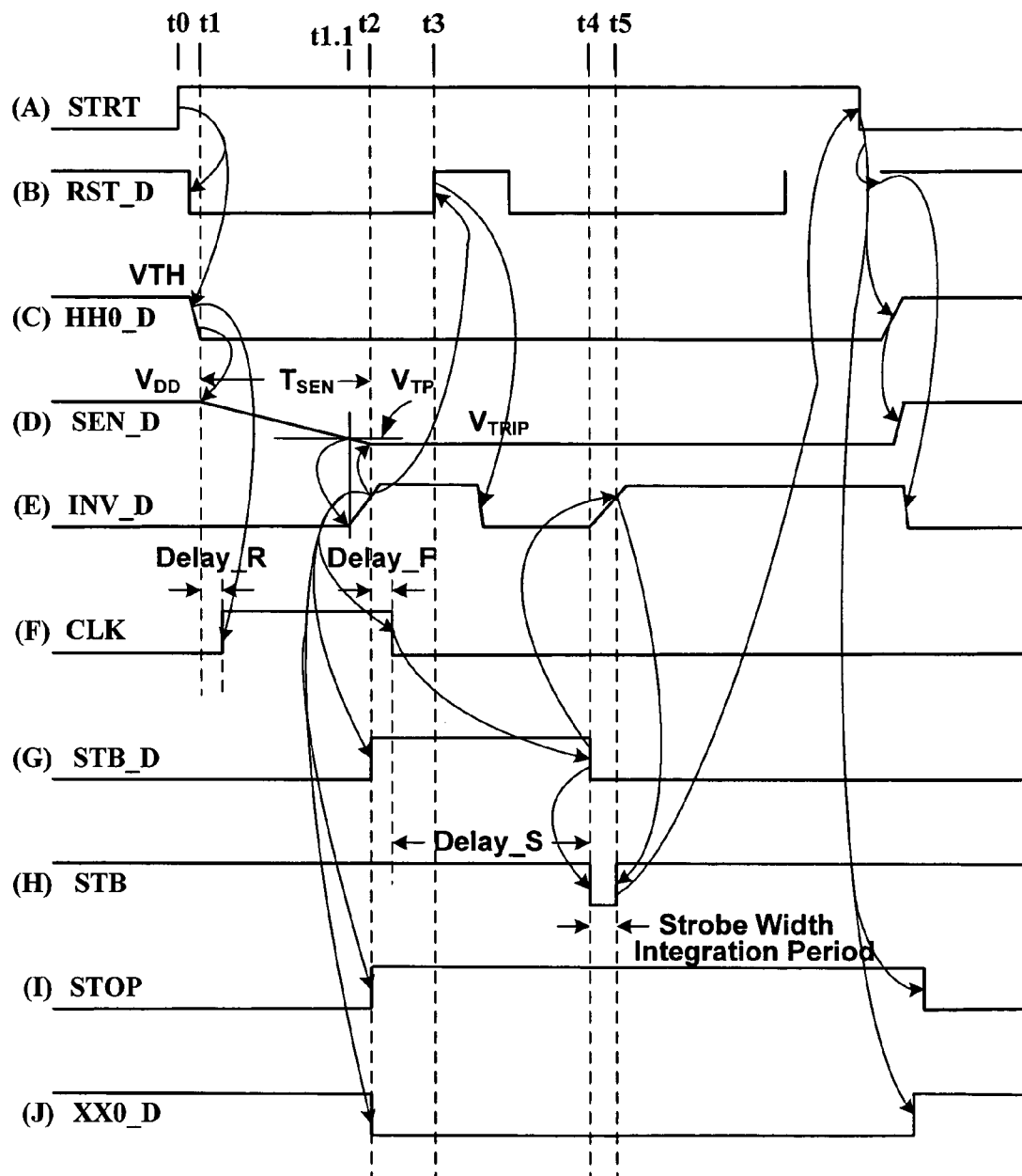
Reference Sense Amplifier's Timing Diagrams
