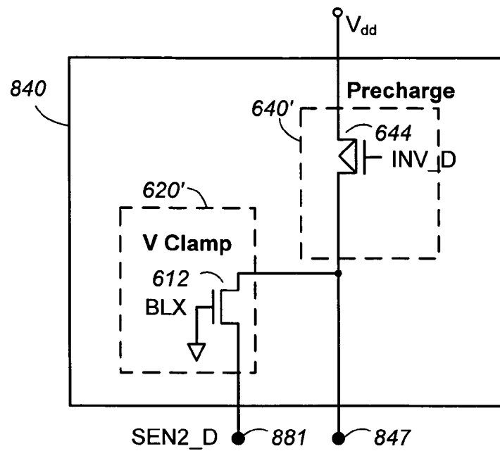
Precharge/Clamp Circuit of Ref Sense Amp
