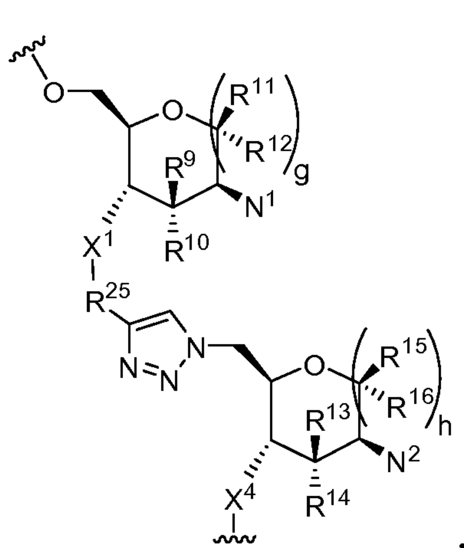
Formula XIa
