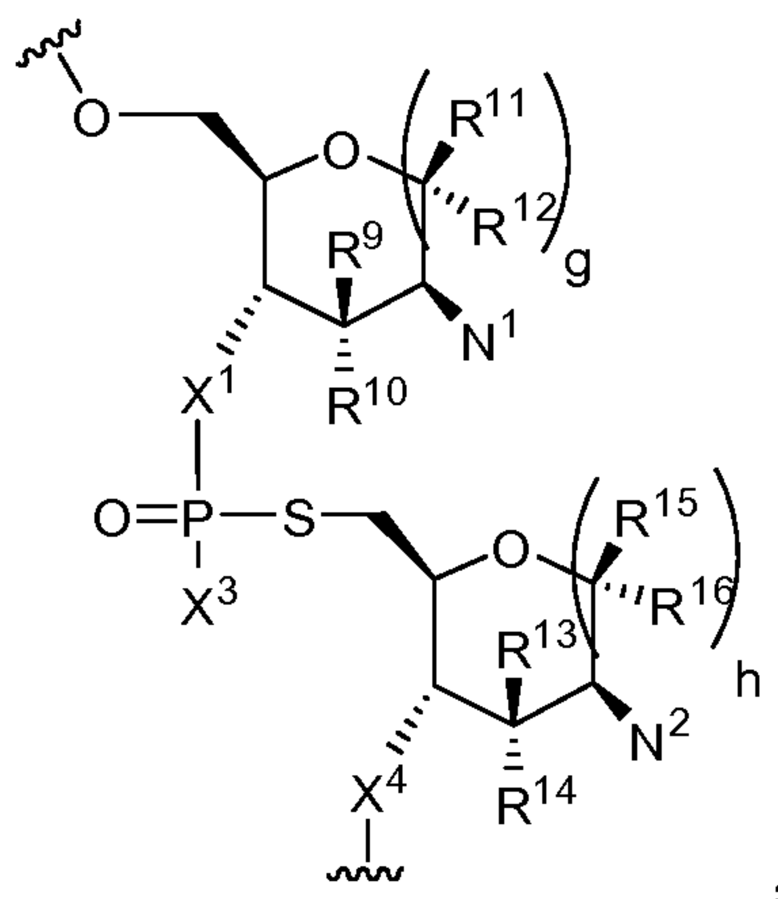
Formula V
