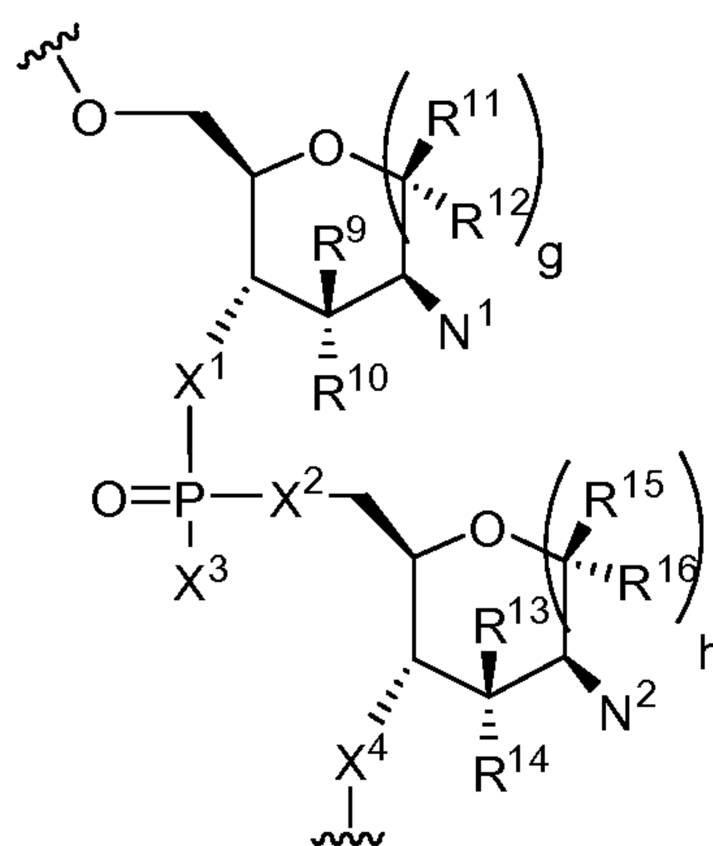
Formula IV
