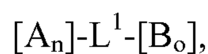
Formula II
