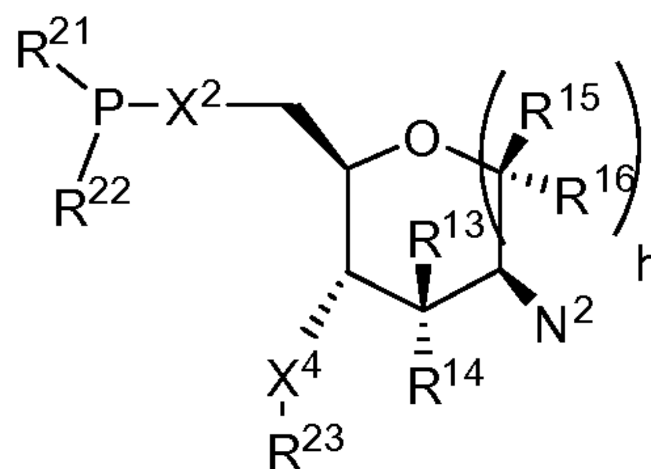
Formula X
