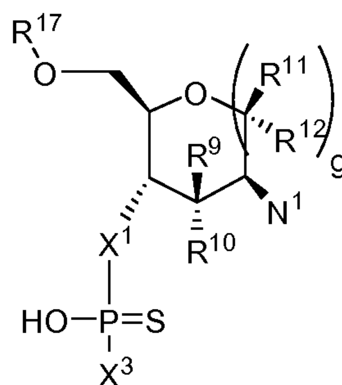
Formula VI
