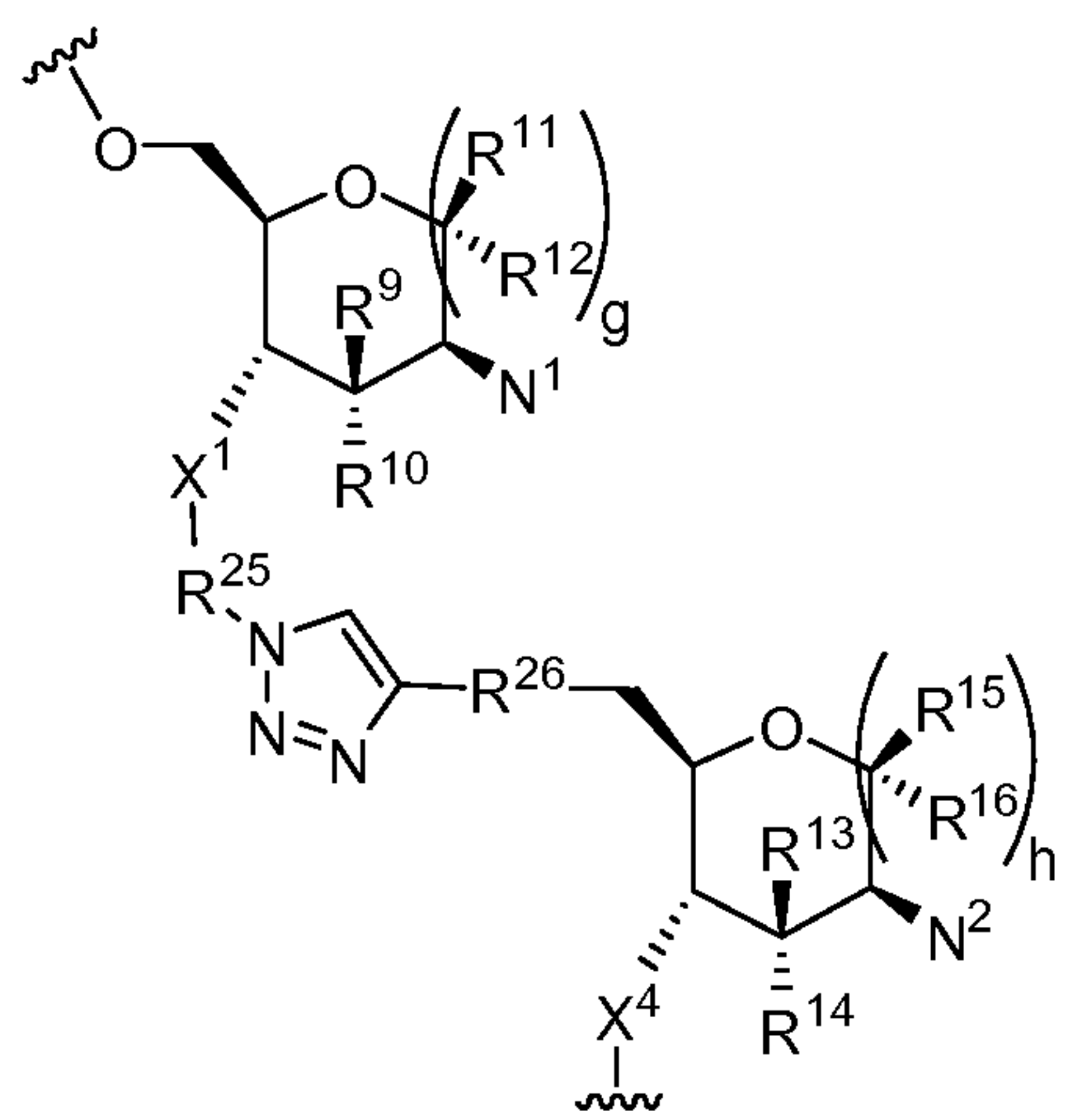
Formula XIb
