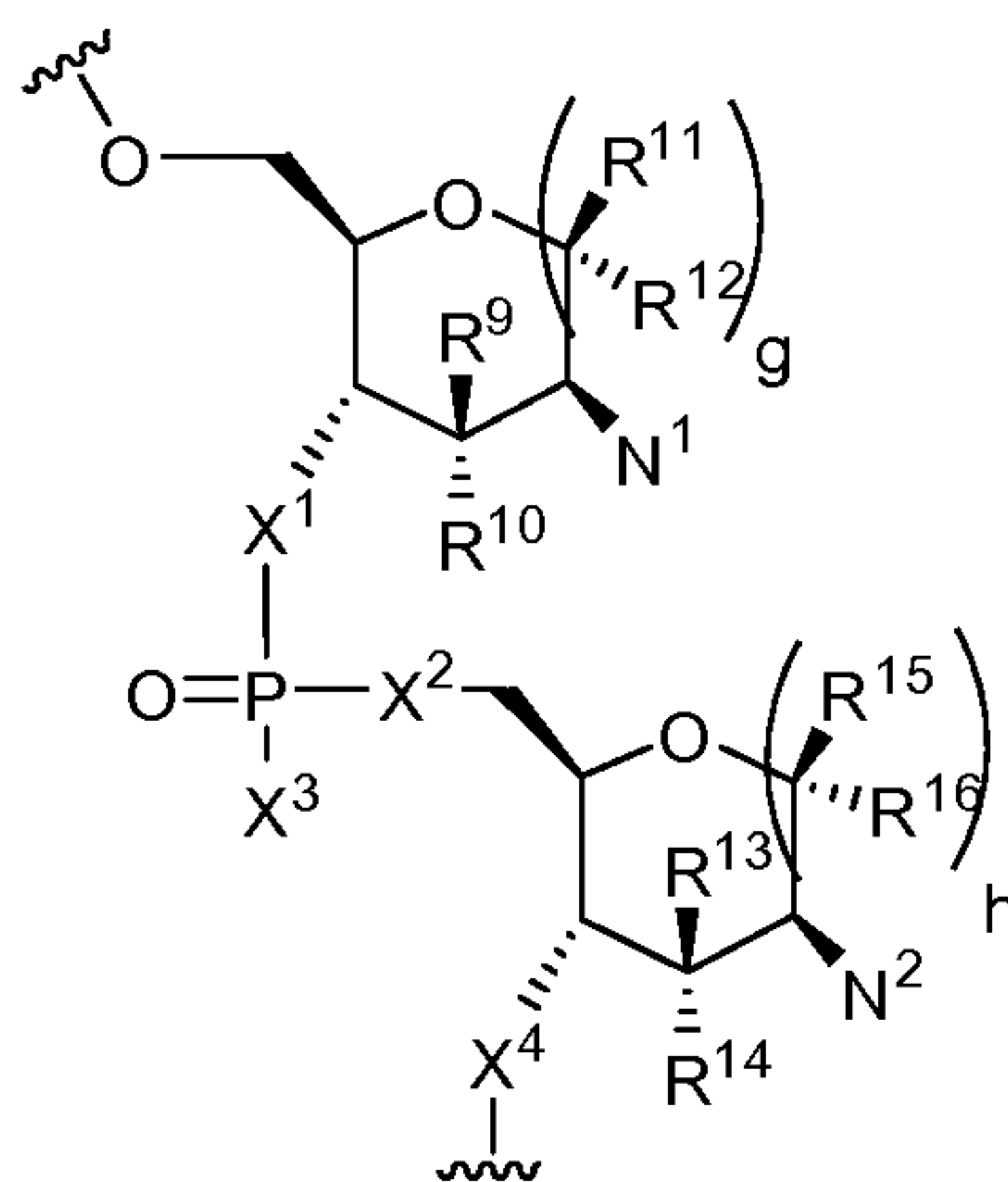
Formula IV
