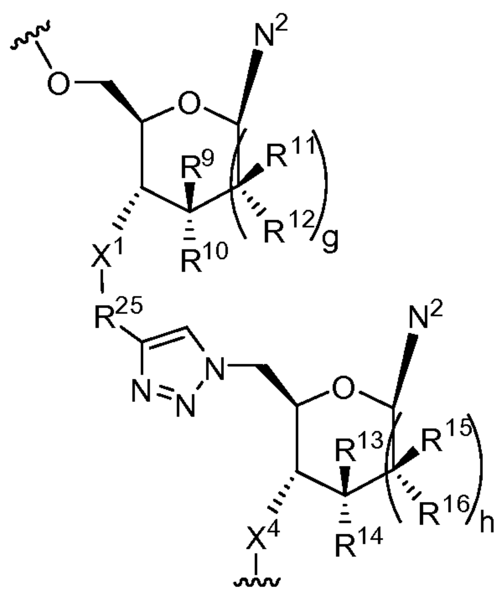
Formula XI
