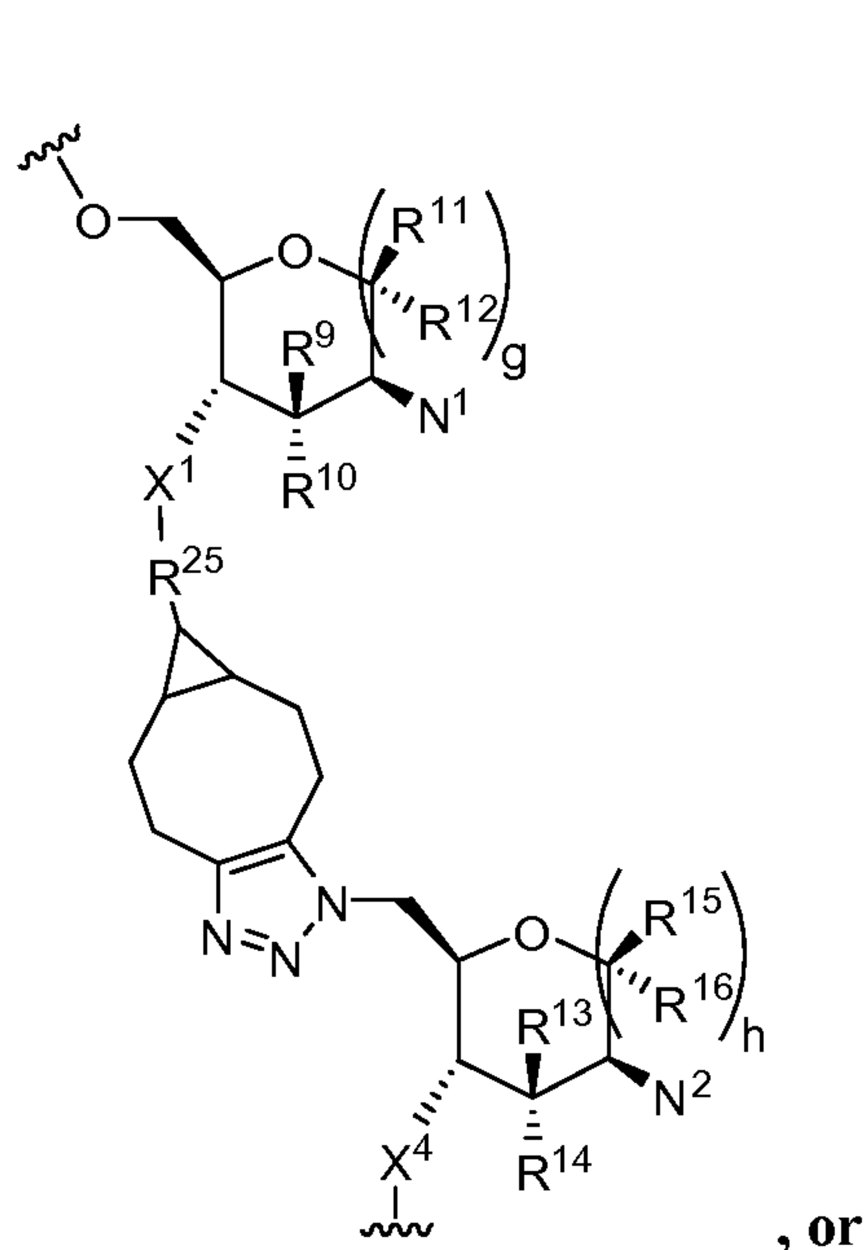
Formula XIa
