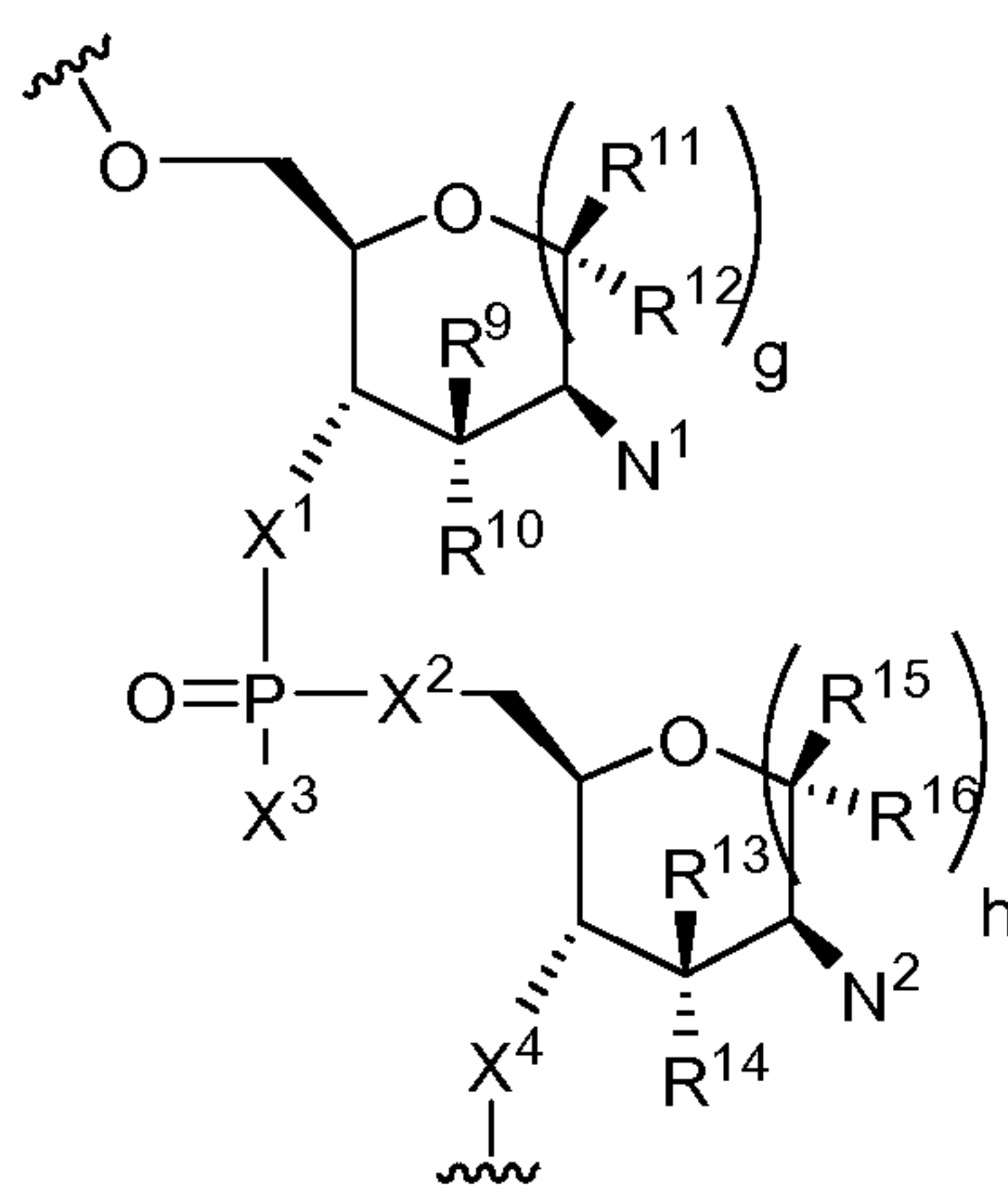
Formula IV
