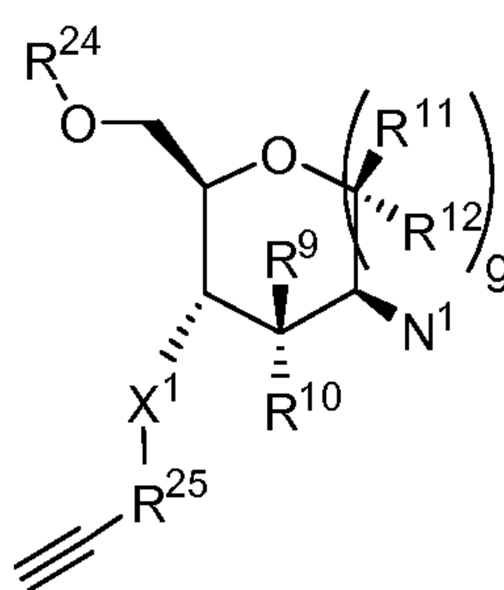
Formula XII
