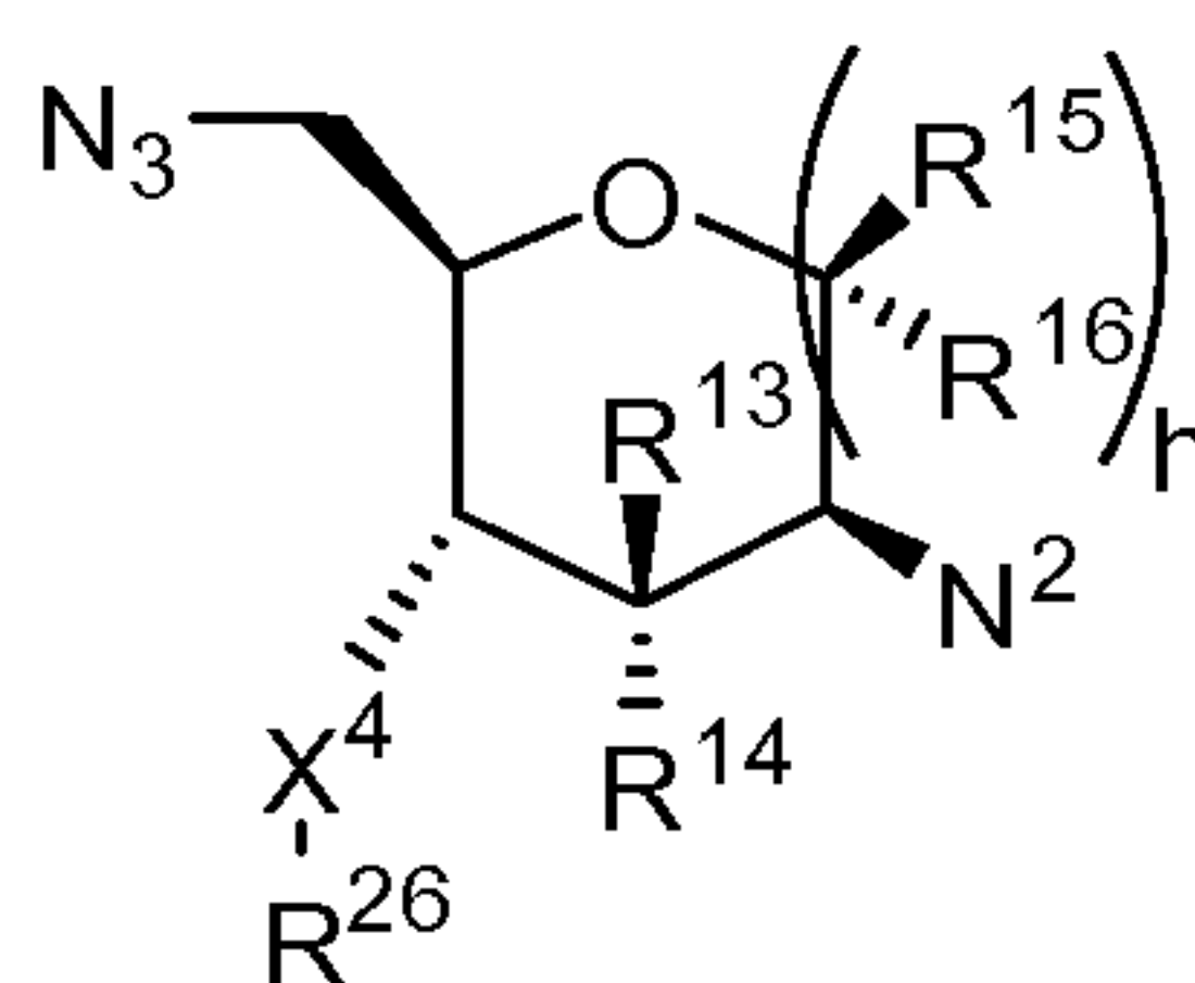
Formula XIII
