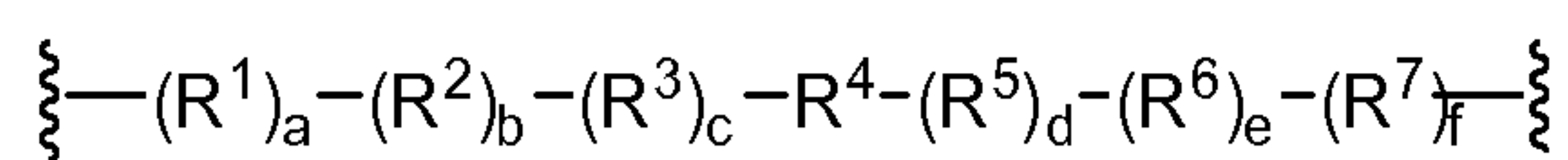
Formula III
