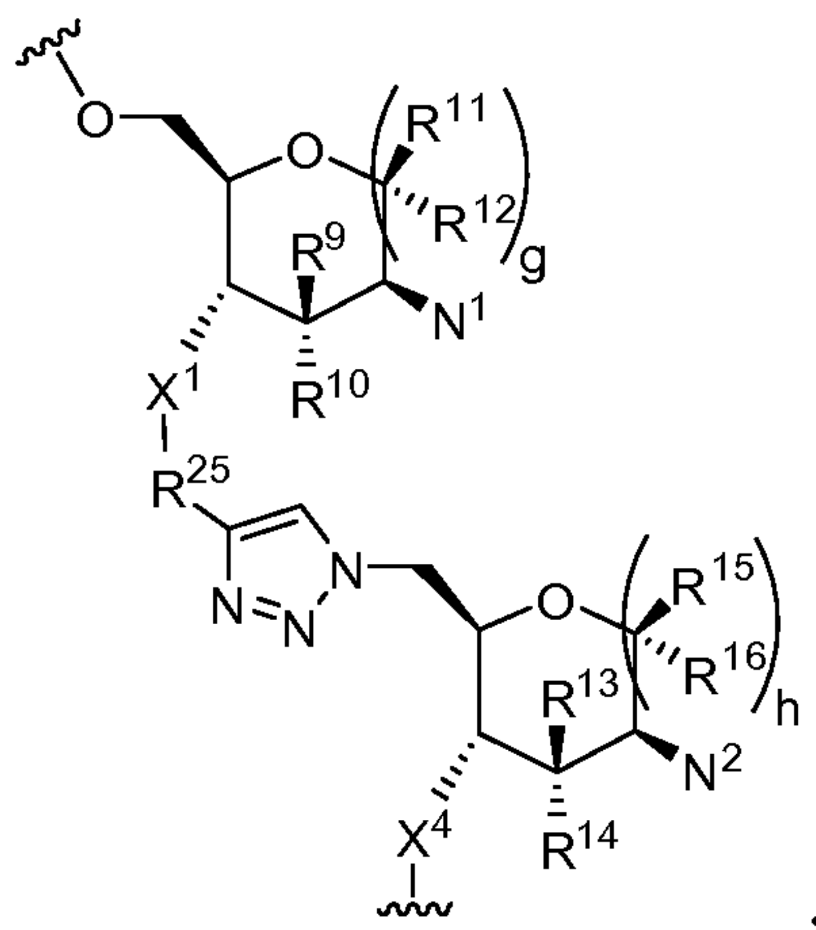
Formula XI
