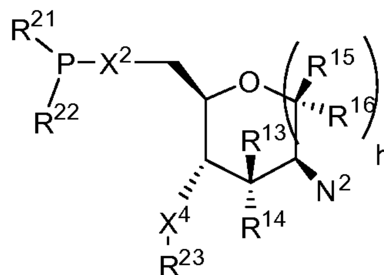
Formula X
