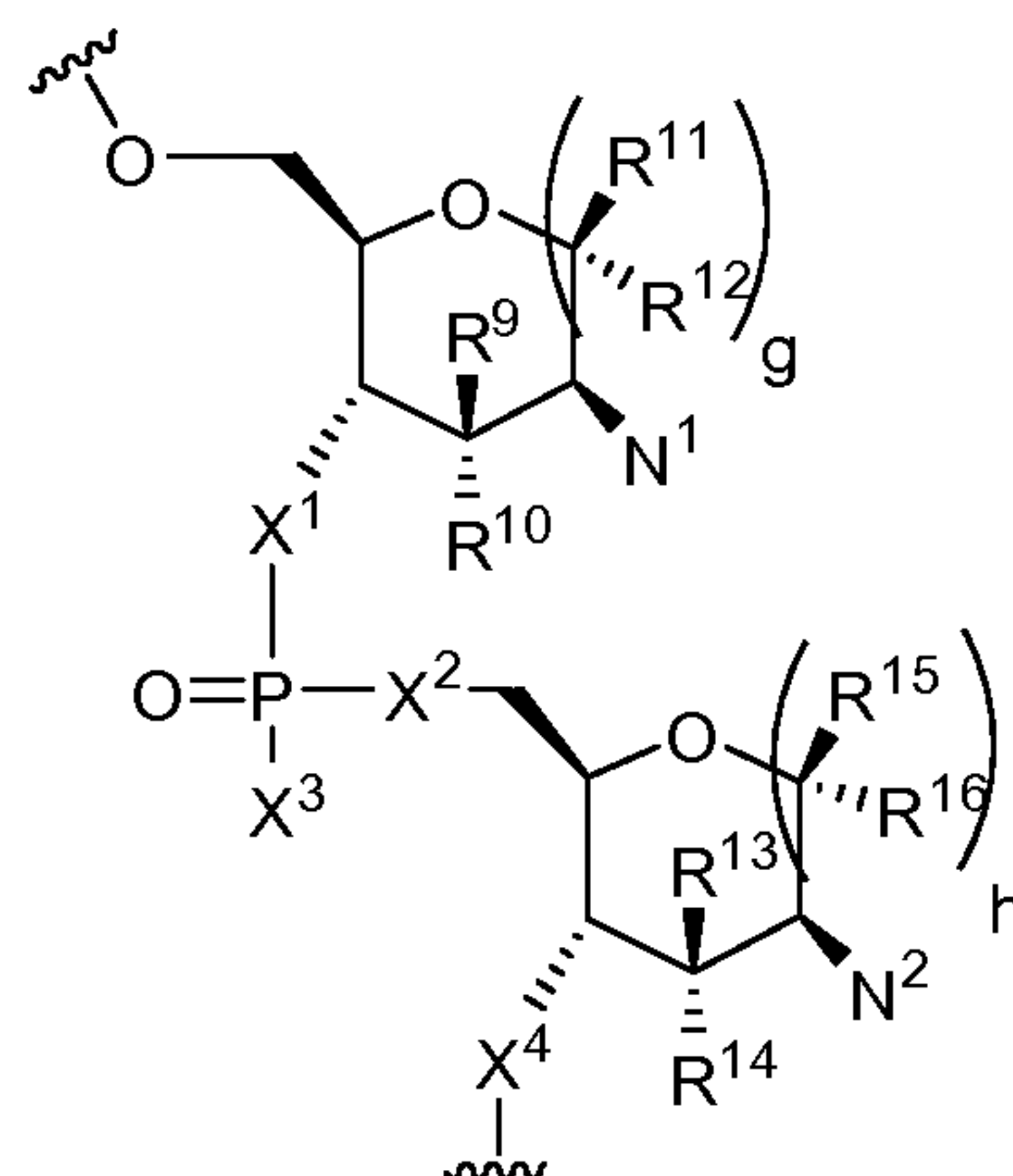
Formula IV
