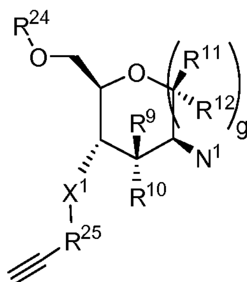
Formula XII
