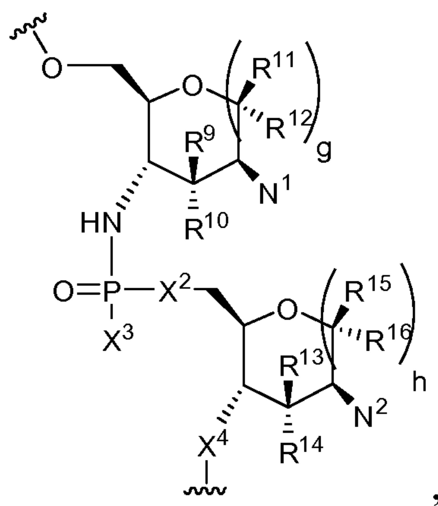
Formula VIII
