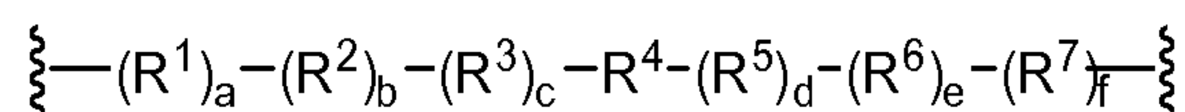
Formula III
