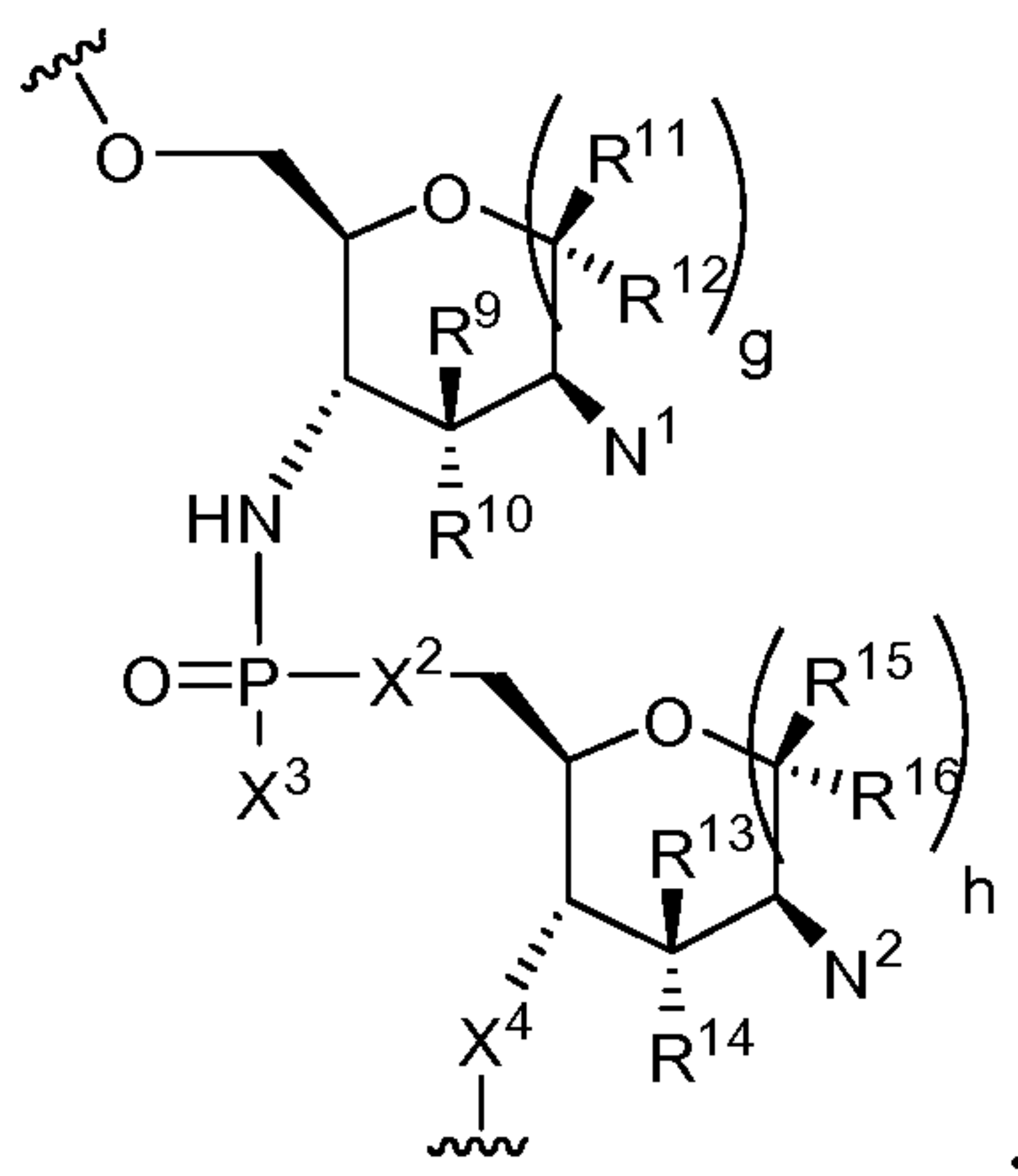
Formula VIII
