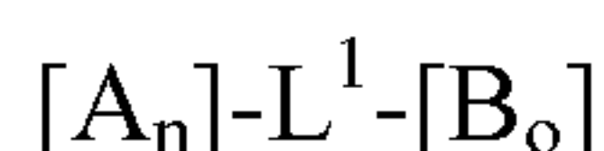
Formula II
