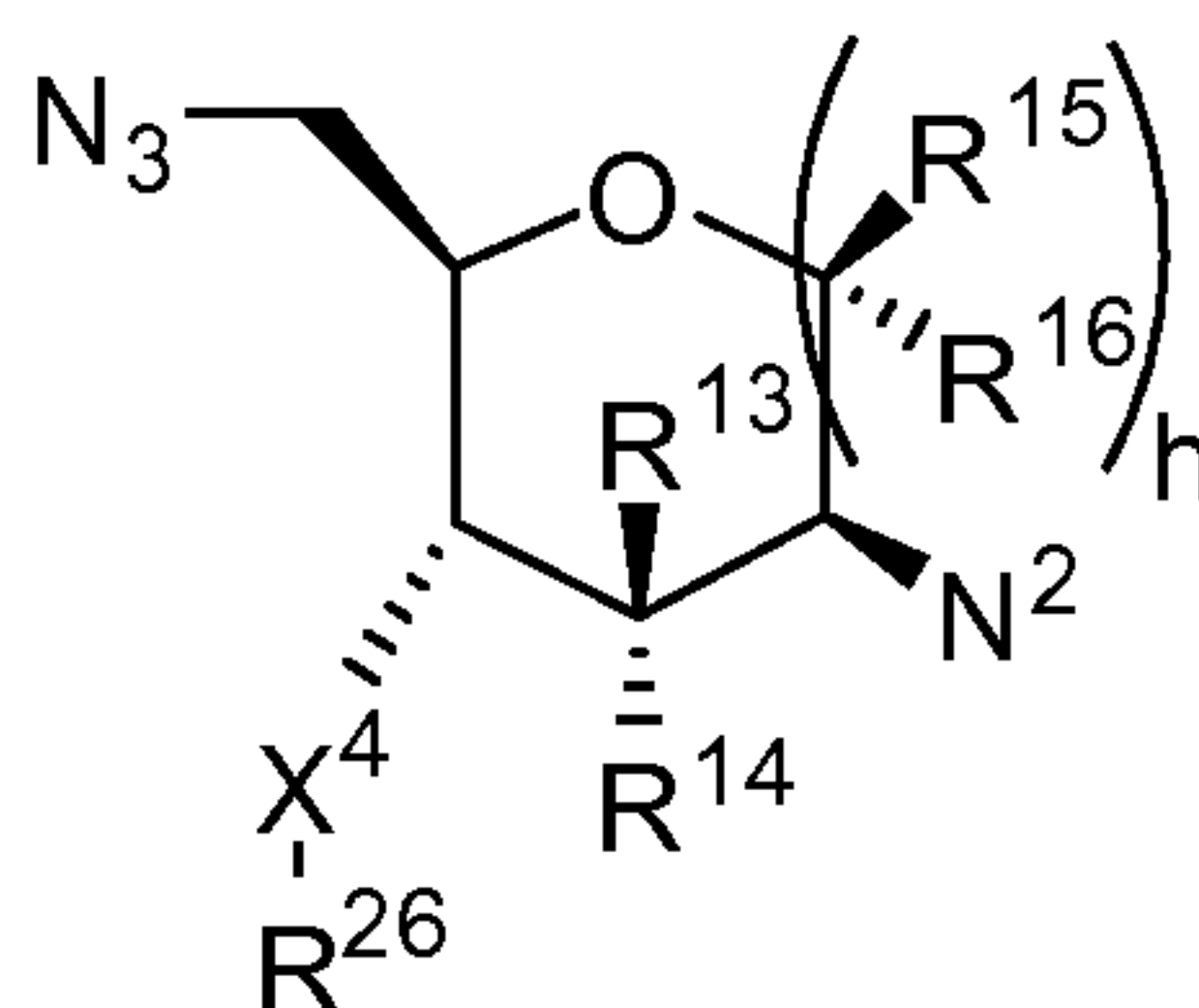
Formula XIII
