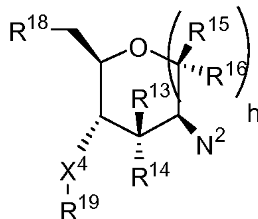
Formula VII
