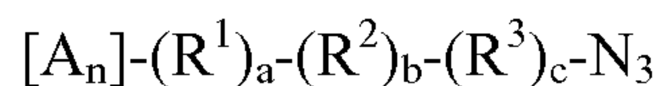
Formula XVI
