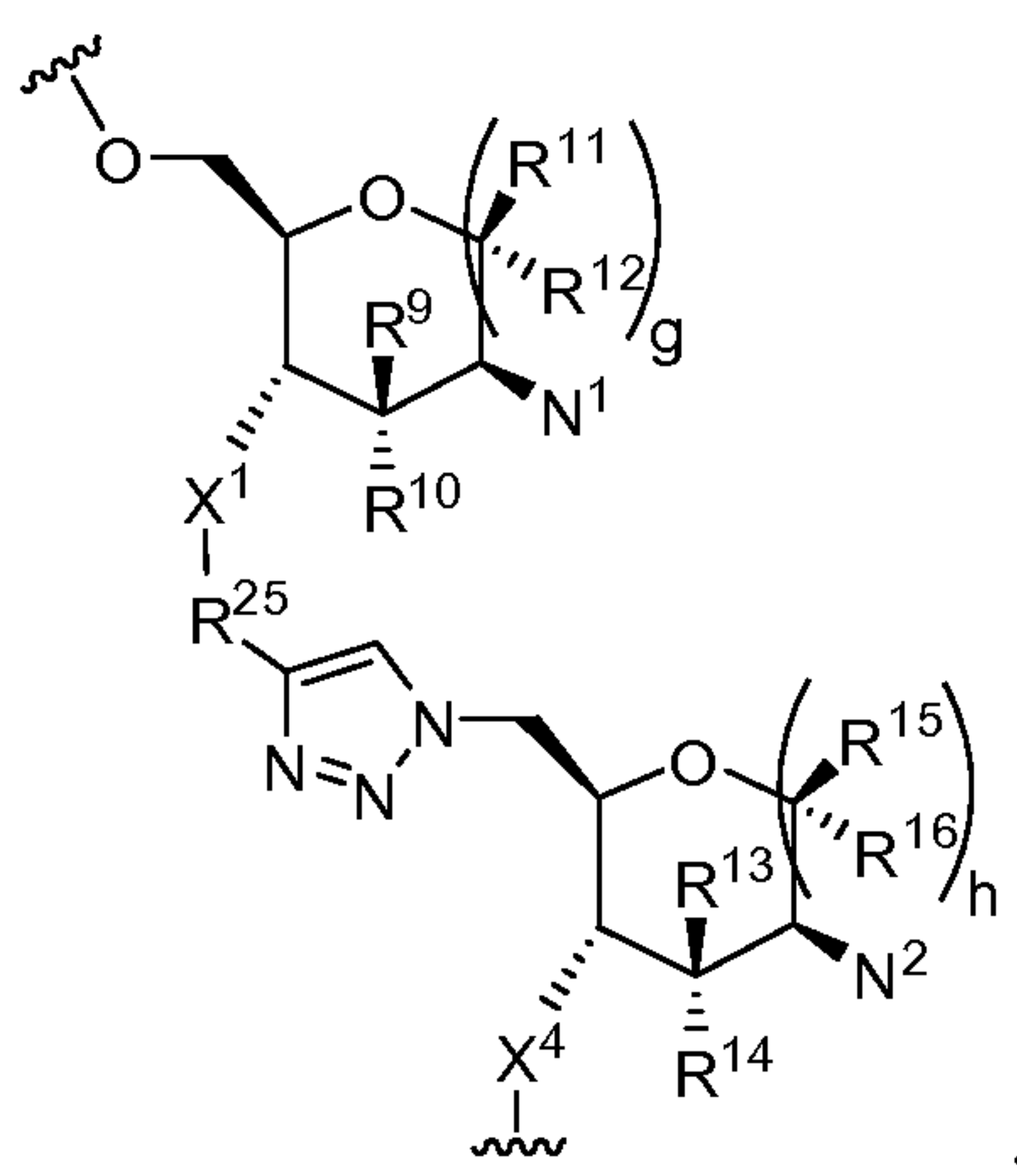
Formula XI
