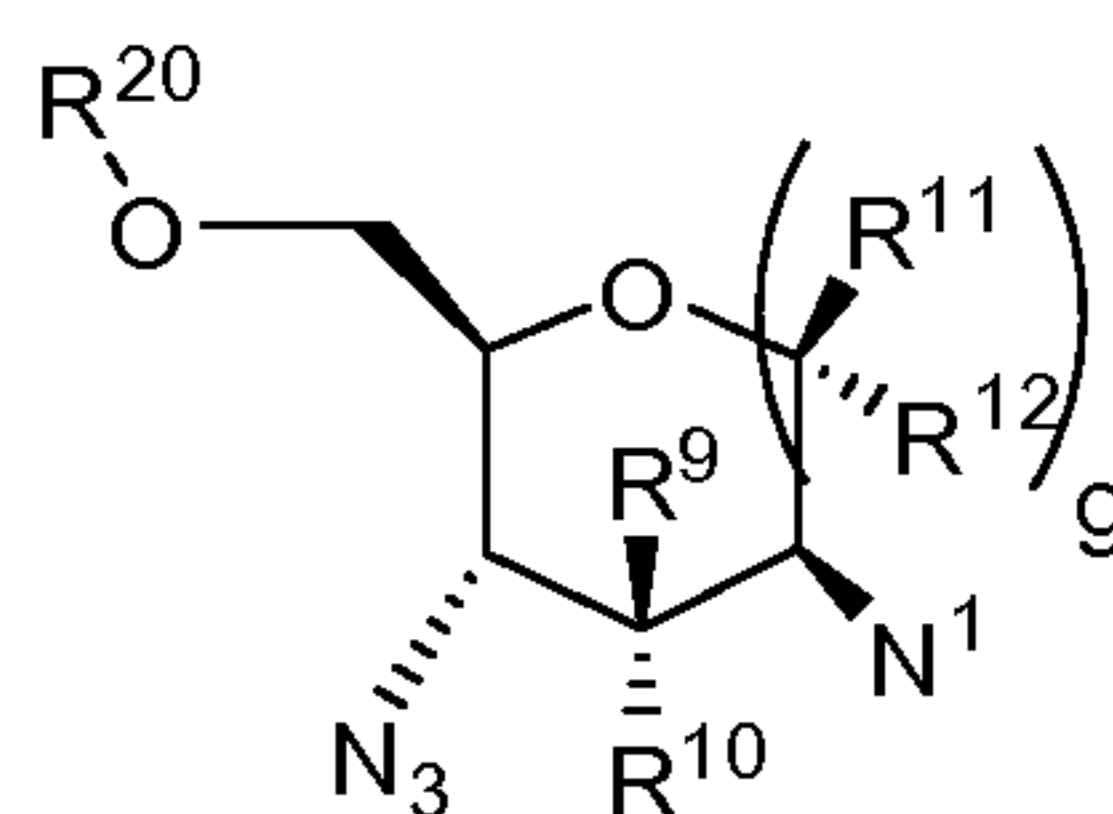
Formula IX
