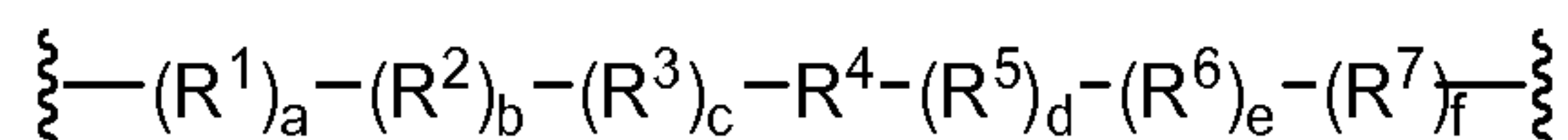
Formula III
