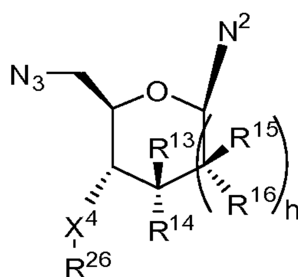
Formula XIII
