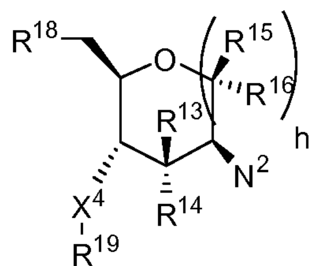
Formula VII
