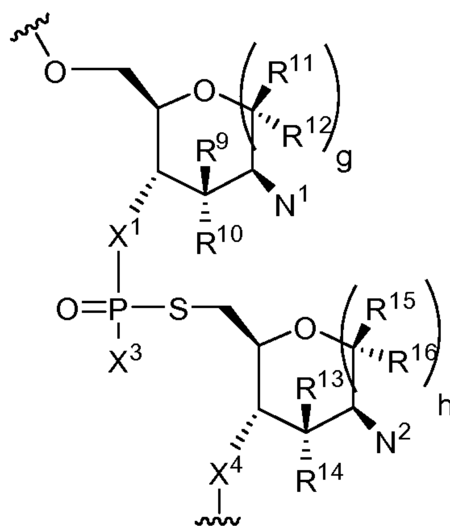
Formula V
