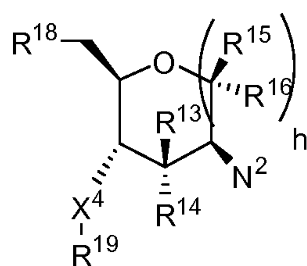
Formula VII
