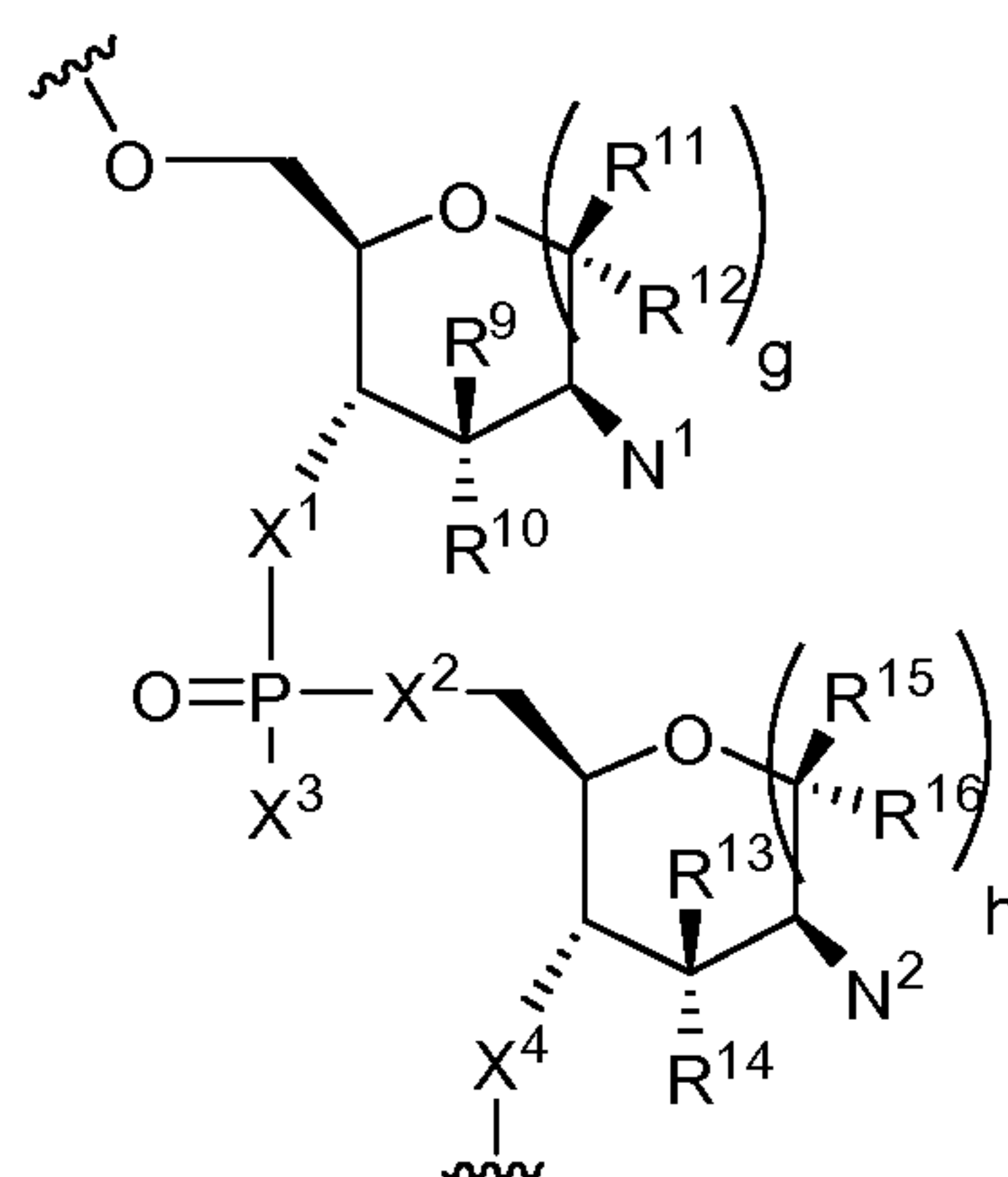
Formula IV
