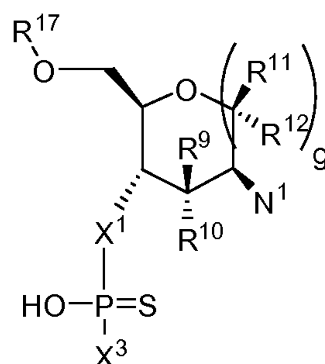
Formula VI
