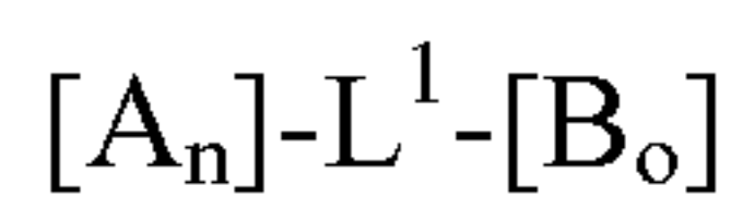
Formula II
