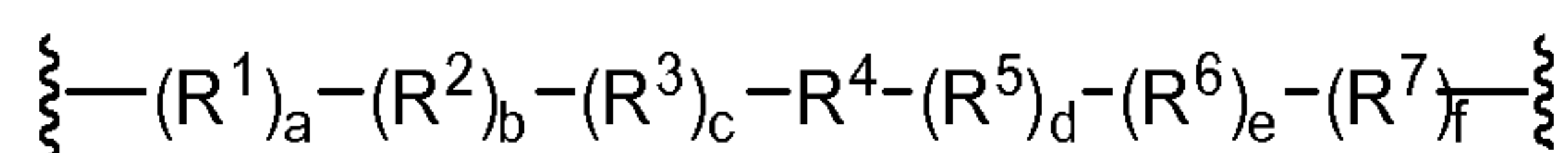
Formula III
