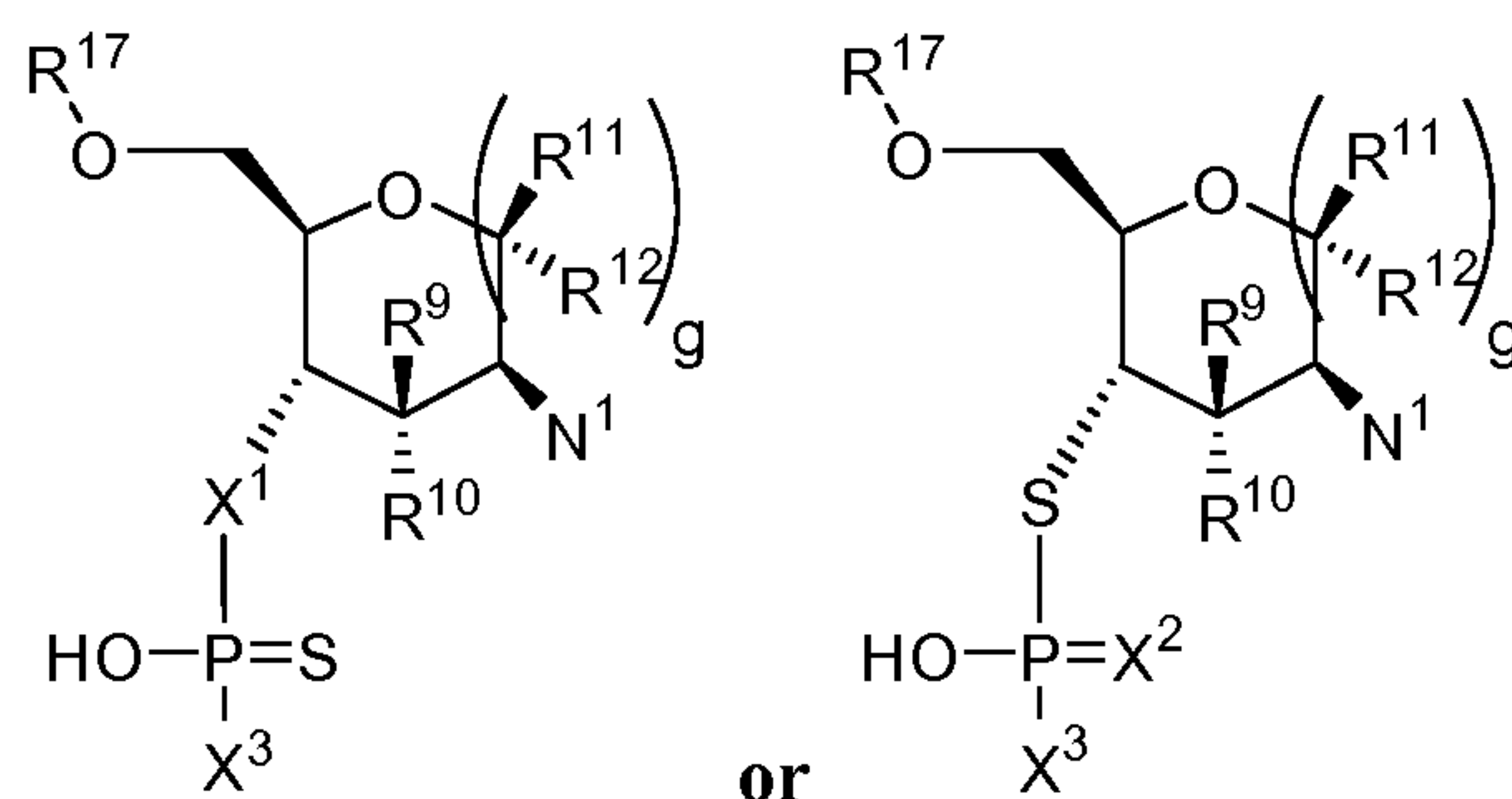
Formula VIa
