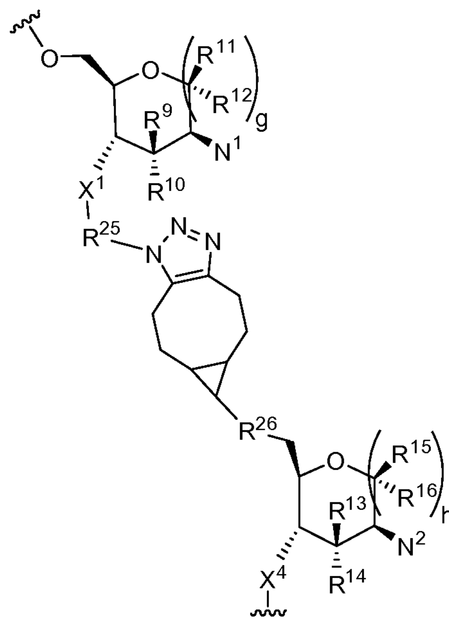
Formula XIb
