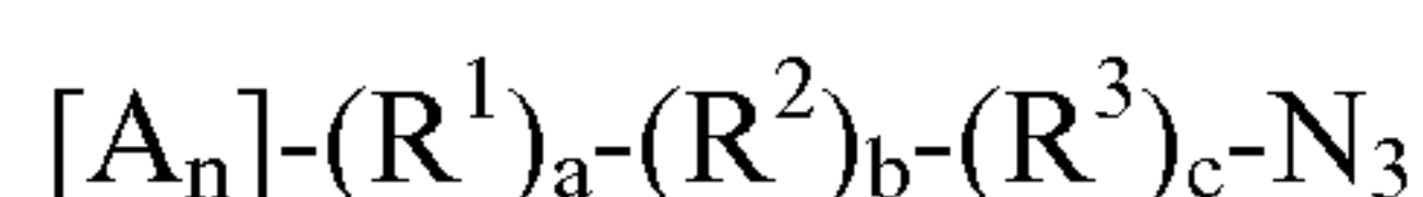
Formula XIV
