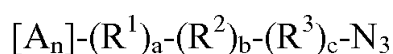
Formula XIV
