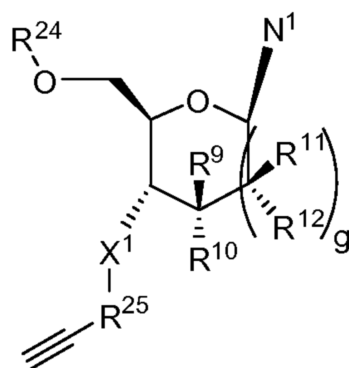
Formula XII
