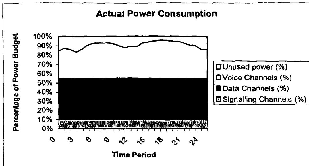
Fig. 3 (Prior Art)
