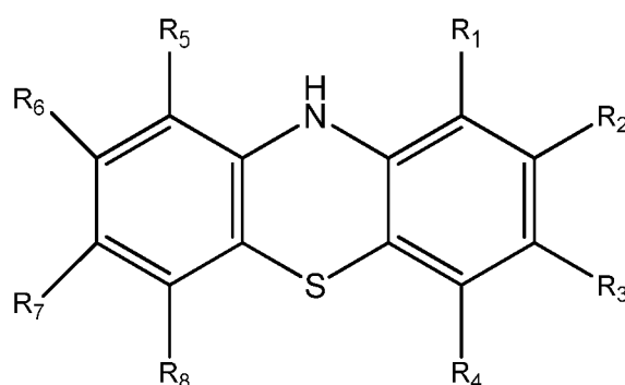
[Chemical Formula 1]
