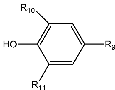
[Chemical Formula 2]
