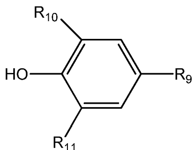
[Chemical Formula 2]
