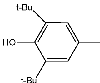
[Chemical Formula 2-1]
