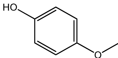
[Chemical Formula 3-1]
