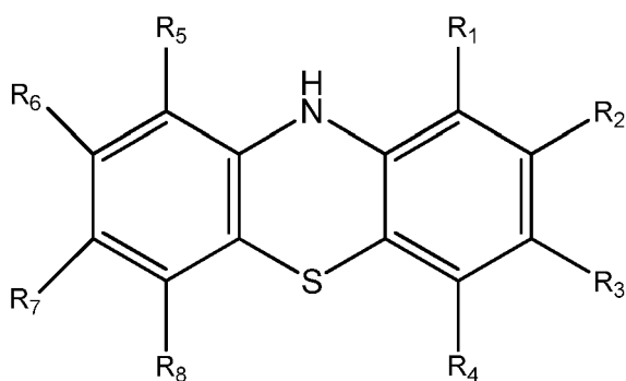
[Chemical Formula 1]
