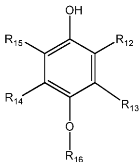
[Chemical Formula 3]
