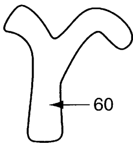
(a) Letter "r"
