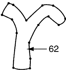
(b) Point Approximation to "r"
