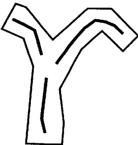
(c) Chordal Axis
