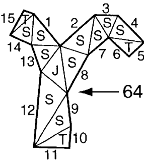
(c) Delaunay Triangulation
