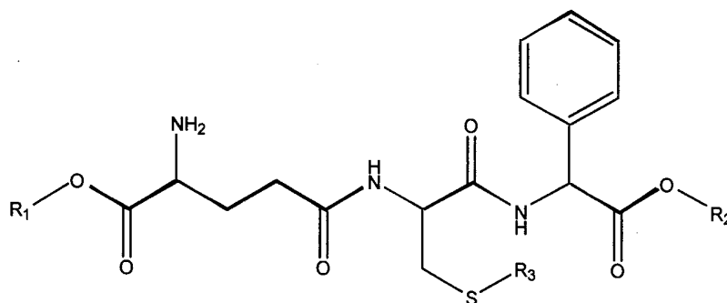
Formula I
