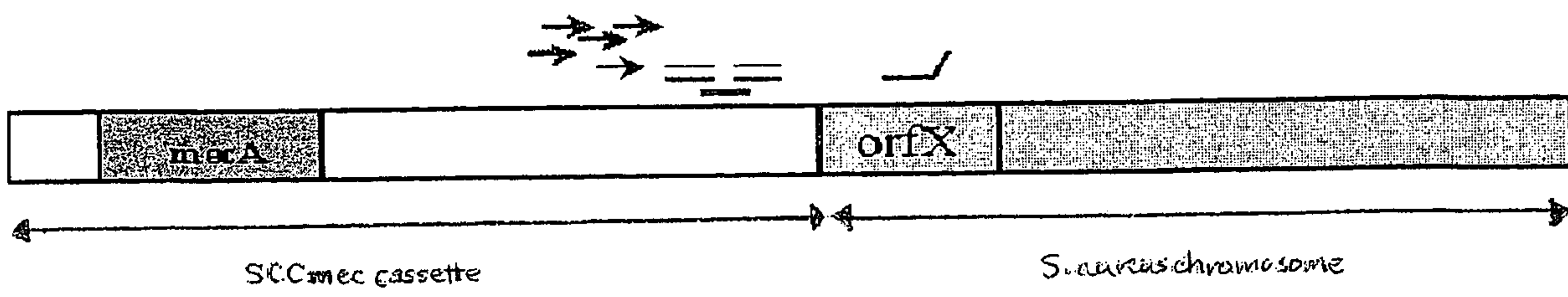
Figure 3 NASBA approach 2
