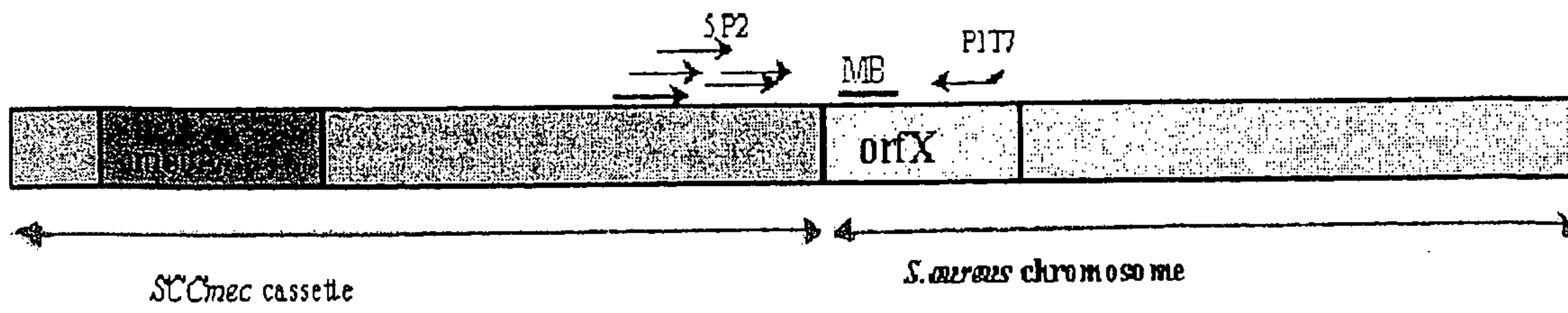
Figure 2 : NASBA approach 1
