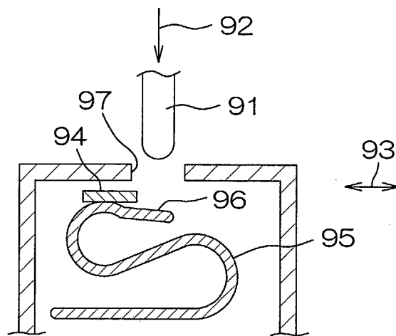
FIG. 12 PRIOR ART
