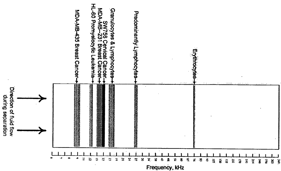
Typical Trapping Profile for Electrosmeared Slides
