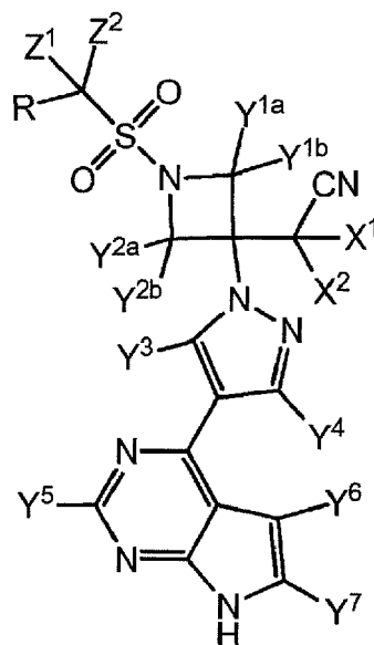
Formula I
