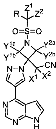
Formula Ia
